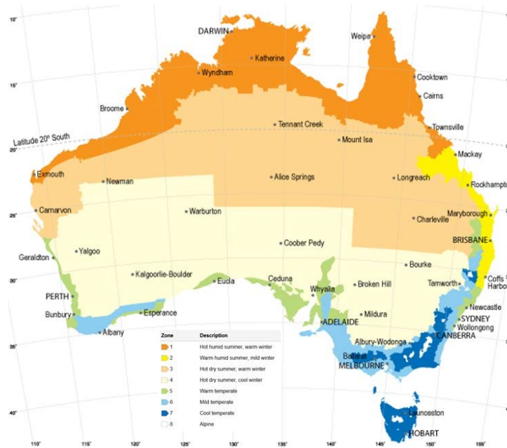
Figure 1: Australian climate zones (ABCB, 2016).
