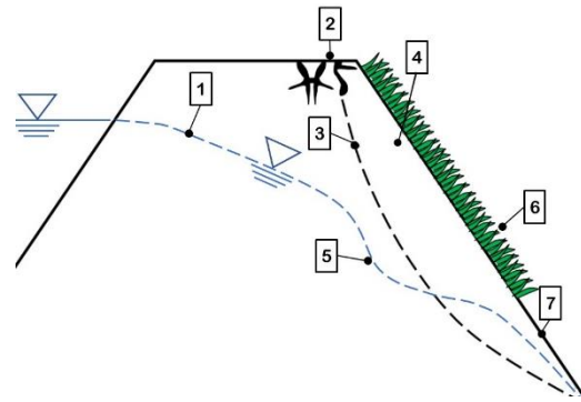
Figure 12. Coupled phenomena in soil-vegetation-atmosphere interactions. 1) Phreatic level affected by soil-atmosphere interactions (drying/wetting cycles). 2) Soil desiccation (shrinkage/cracking and effects on infiltration and landslide initiation). 3) Slope stability (soil cracking and vegetation effects on soil hydro-mechanical behaviour). 4) Vegetation features (root/soil ratios, depth, morpho-physiology) and vegetation growth/decay (water retention curve, permeability, microstructure, volume change and shear strength properties, carbon sequestration, mucilage chemical effect). 5) Vegetation-induced suction ('capillary barrier effect, mechanical strengthening, effect on slope stability). 6) Soil-vegetation-atmosphere interactions (evapotranspiration, leaf coverage). 7) Soil erosion and runoff velocity.
