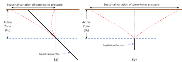
Figure 22. (a) Concept of equilibrium suction profile (b) Concept of equilibrium suction for regions with deep or absent phreatic level
