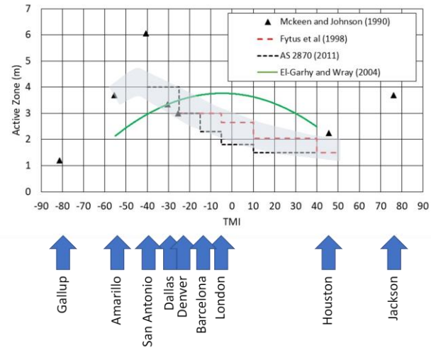
Figure 21. Association between TMI and active zone depth.
