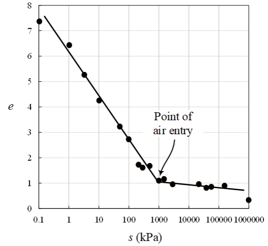
Figure 8. Mechanical response of a normally consolidated soil subjected to increasing values of suction – experimental data (data from Fleureau et al 1993).
