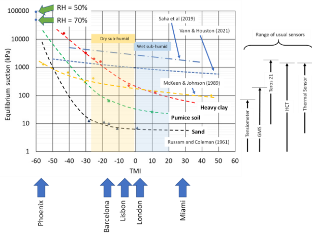
Figure 23. Relationship between equilibrium suction and TMI.
