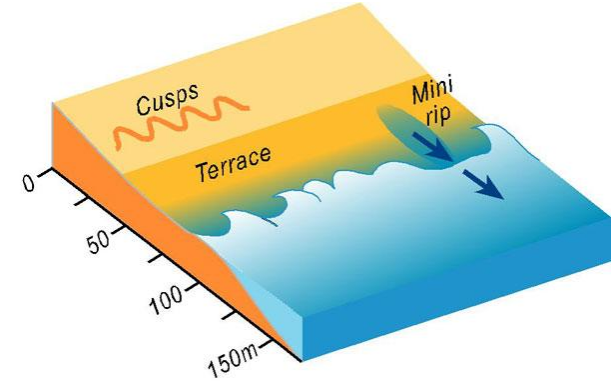
Type 5 Low Tide Terrace
