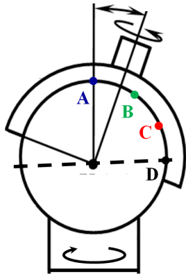
Fig. 4 A spherical polishing system with three independent angular velocities.
