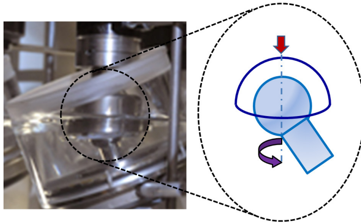
Fig. 3 The motion in a hip joint simulator (left image: https://www.beaumont-hospitals.com ).
