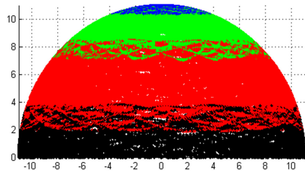
Fig. 5 The combined trajectories of cutting edges A, B, C and D in Fig. 4 on the sphere subjected to polishing [41].
