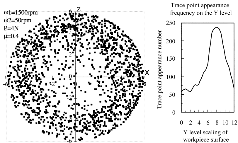
Fig. 17. The polishing trace on the workpiece surface ( \omega_1=1500\text{ rpm} ).
