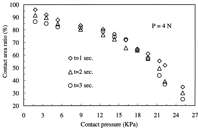
Fig. 7. Relation between contact area ratio and contact pressure.
