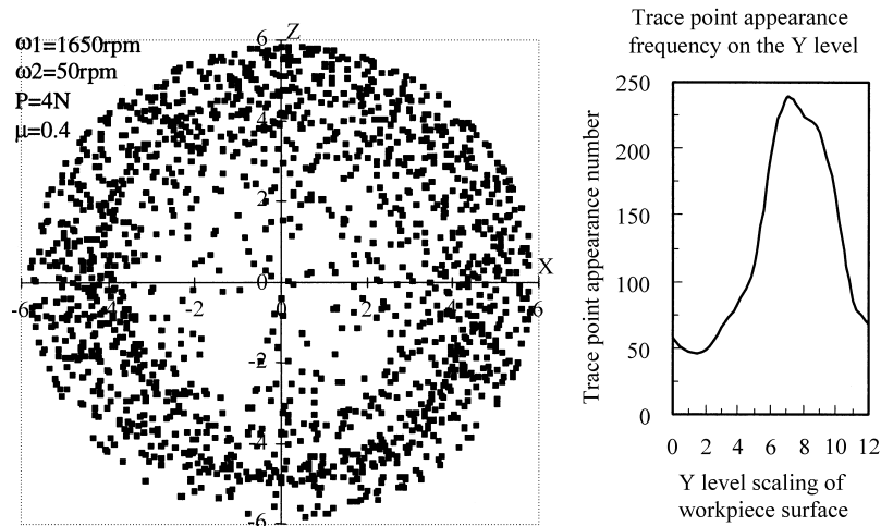
Fig. 18. The polishing trace on the workpiece surface ( \omega_1=1650 rpm).
