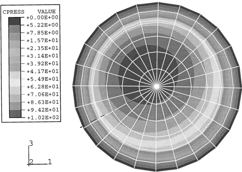
Fig. 3. Polishing pressure distribution at t=0.1 s.
