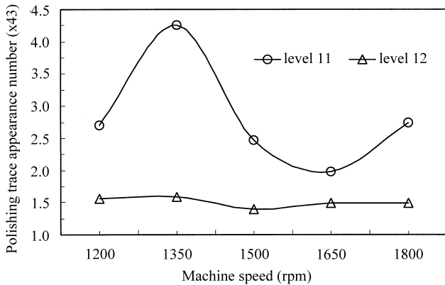
Fig. 21. Trace distribution analysis on edge area of workpiece surface.
