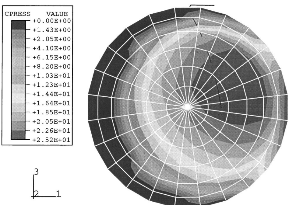
Fig. 4. Polishing pressure distribution at t=1.0 s.
