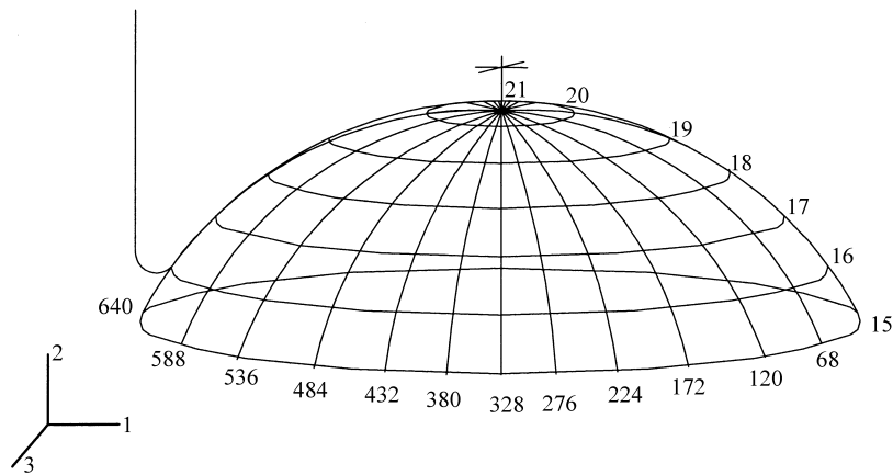
Fig. 2. Mesh of modelled contact surface.
