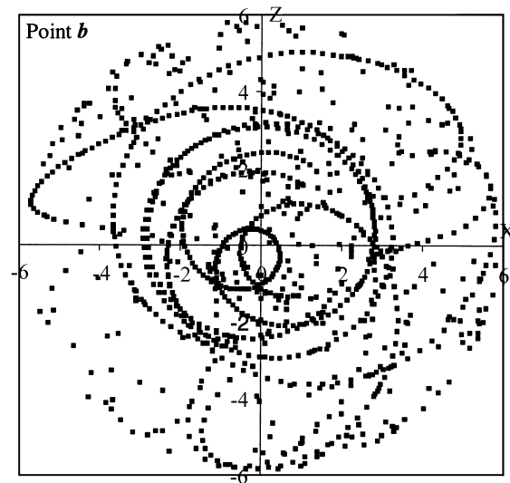
Fig. 10. The polishing trace pattern on the workpiece surface created by point b .
