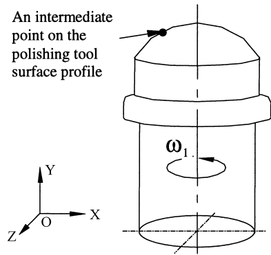
Fig. 14. Illustration of an intermediate point on the polishing tool surface.
