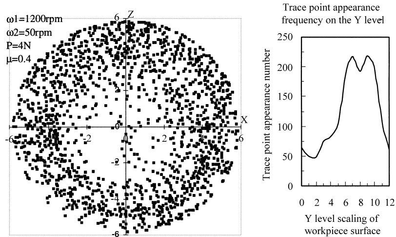
Fig. 15. The polishing trace on the workpiece surface ( \omega_1=1200\text{ rpm} ).
