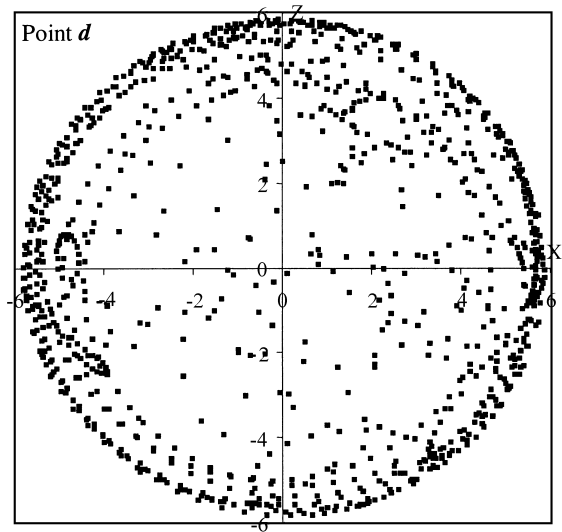
Fig. 12. The polishing trace pattern on the workpiece surface created by point d.
