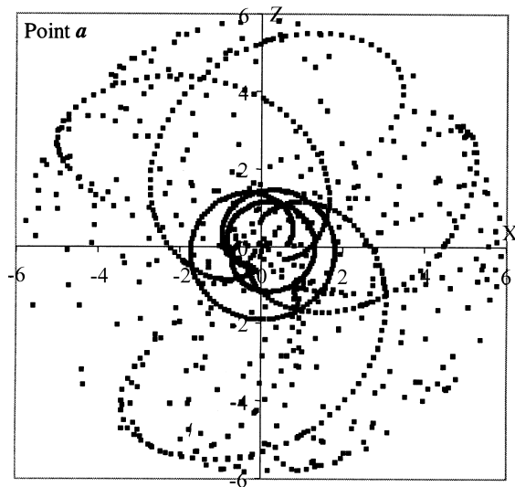
Fig. 9. The polishing trace pattern on the workpiece surface created by point a .
