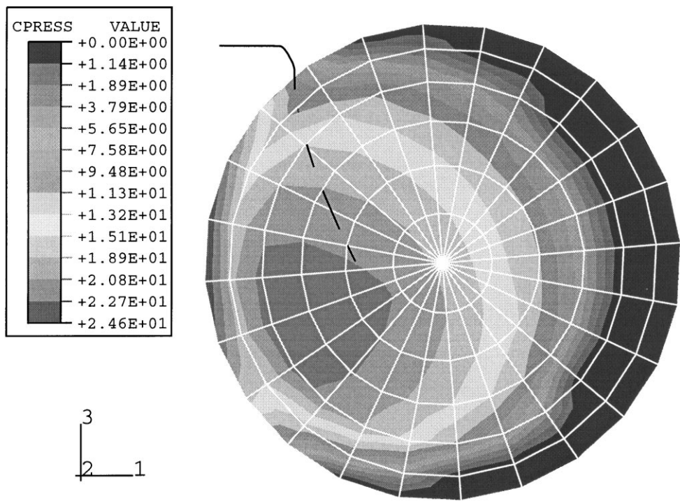
Fig. 5. Polishing pressure distribution at t=2.0 s.
