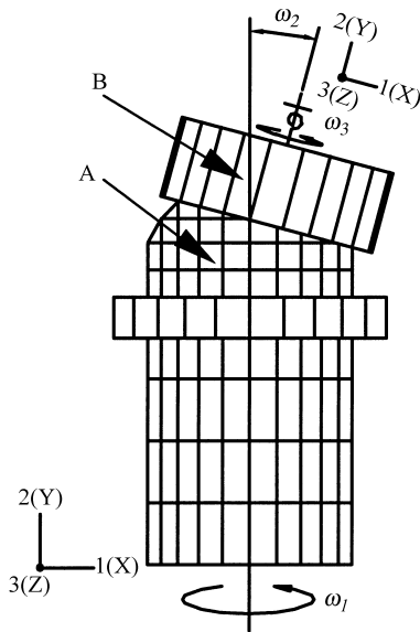
Fig. 1. Illustration of the polishing process.
