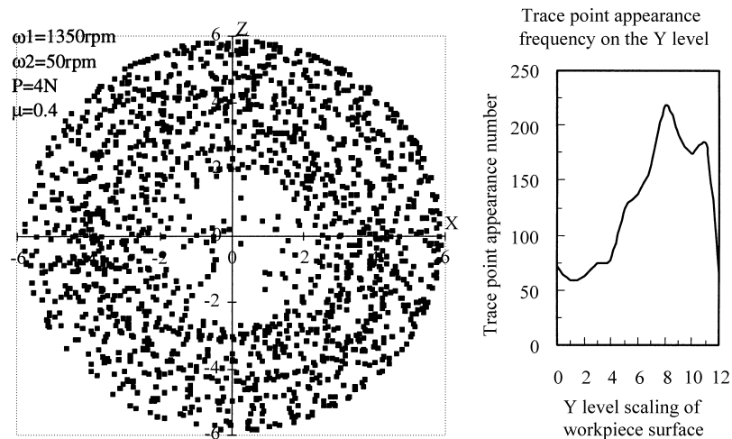
Fig. 16. The polishing trace on the workpiece surface ( \omega_1=1350\text{ rpm} ).
