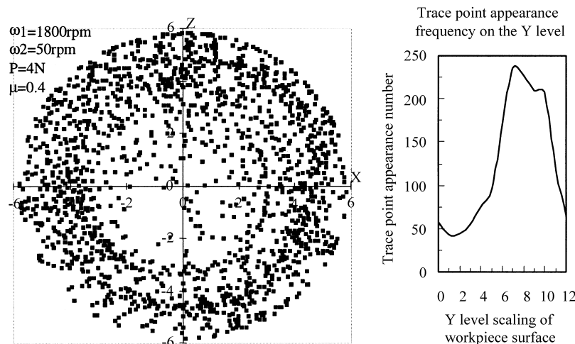
Fig. 19. The polishing trace on the workpiece surface ( \omega_1=1800 rpm).
