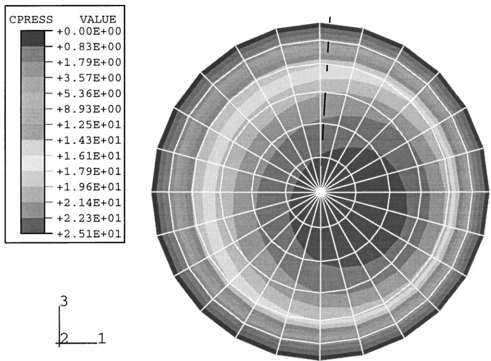
Fig. 6. Polishing pressure distribution at t=3.0 s.
