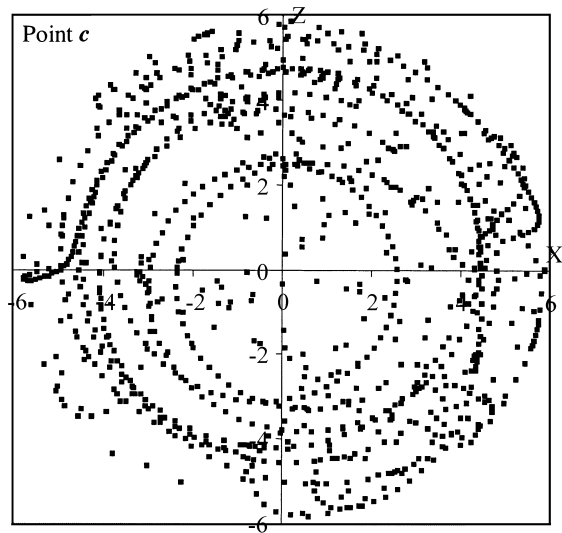
Fig. 11. The polishing trace pattern on the workpiece surface created by point c.
