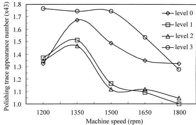
Fig. 20. Trace distribution analysis on centre area of workpiece surface.
