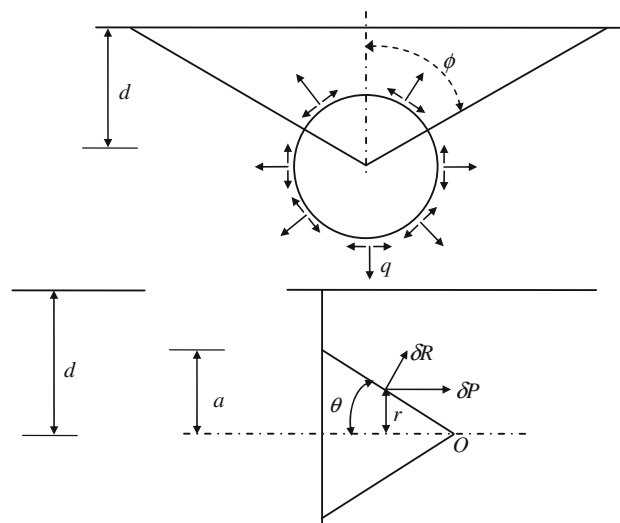
Fig. 1 The schematic diagrams of forces used by Evans 1984
