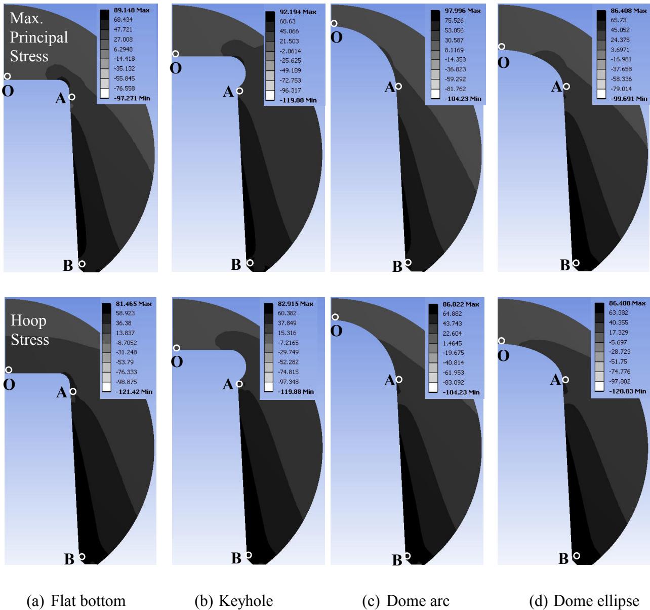
Fig. 3 Contour plots of stresses in ceramic femoral head with four borehole shapes
