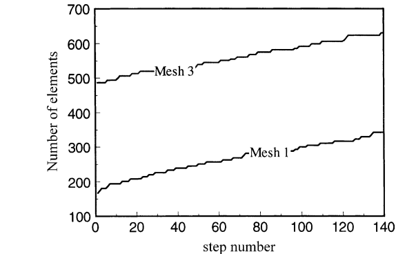
Fig. 4. Total number of elements and remeshing.
