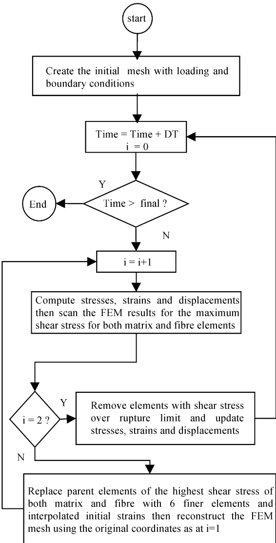
Fig. 5. The adaptive algorithm of remeshing for cutting simulation.
