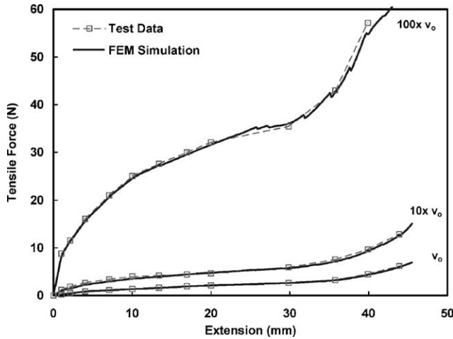
Fig. 11. Tensile forces in bias tension tests. Comparison between experimental data and FEM predictions based on the restrained membrane model.
