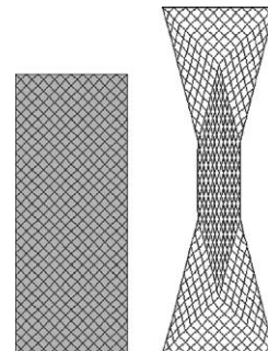
Fig. 10. Initial and deformed mesh profiles in bias tension test simulations.
