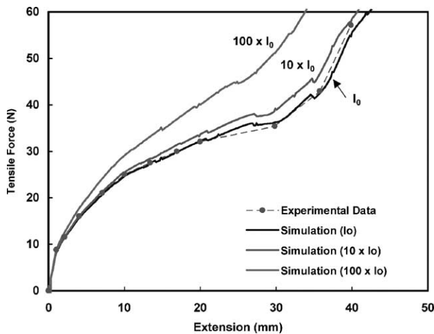
Fig. 15. Effects of fibre in-plane bending stiffness on simulated tensile forces.
