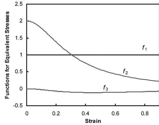
Fig. 13. Functions used to calculate equivalent von Mises stresses for an IFRF model with anisotropic viscous fluid.
