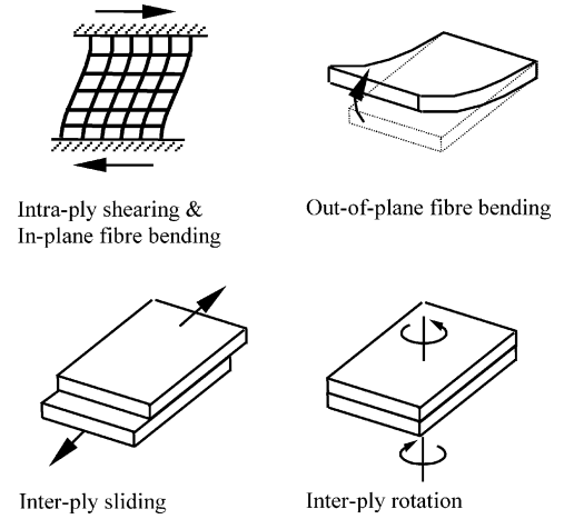
Fig. 2. Predominant intra-ply and inter-ply deformation mechanisms in diaphragm forming process.
