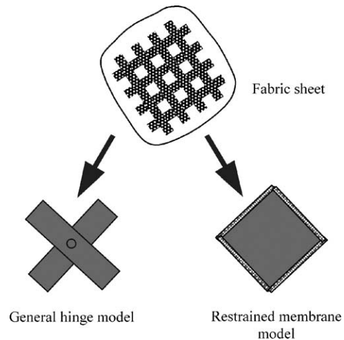
Fig. 6. Illustrations of intra-ply shearing models for FEM analysis.
