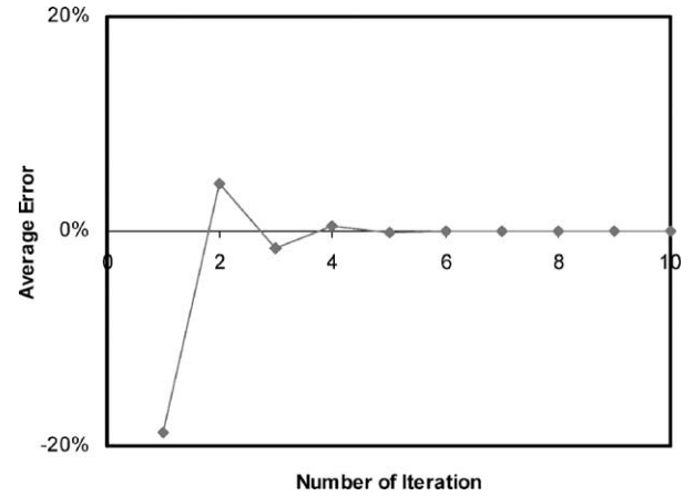
Fig. 8. The convergence of material property determination by the iteration approach.
