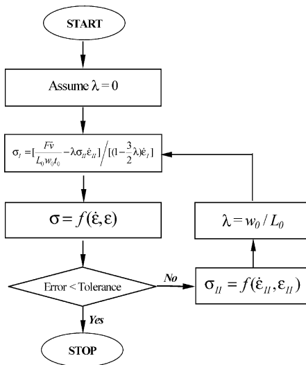
Fig. 7. A flow chart showing iteration approach to determine material properties from bias tension tests.
