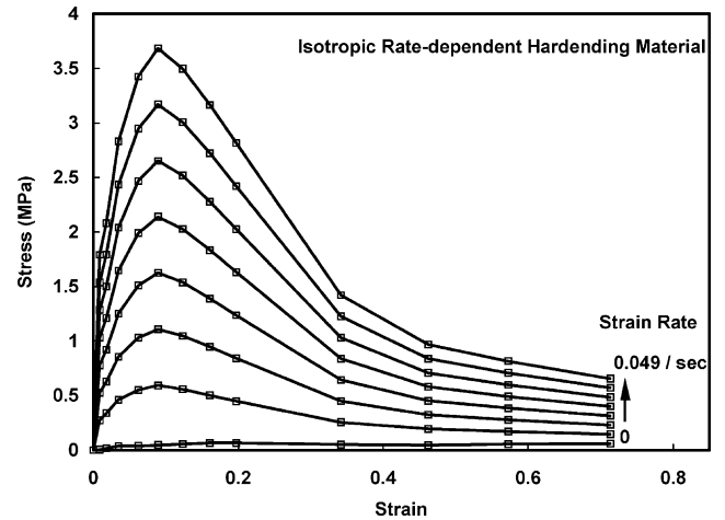
Fig. 9. The material properties of restrained membrane for equivalent simulations of intra-ply shearing stiffness.
