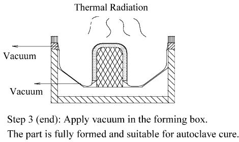
Fig. 1. Schematic illustrations of the double-diaphragm forming process (after [1]).
