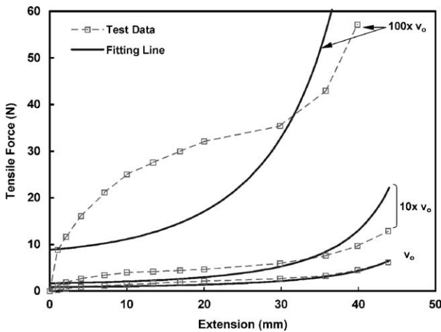
Fig. 5. Tensile forces in bias tension tests. Comparison between experimental data and the IFRF model predictions.
