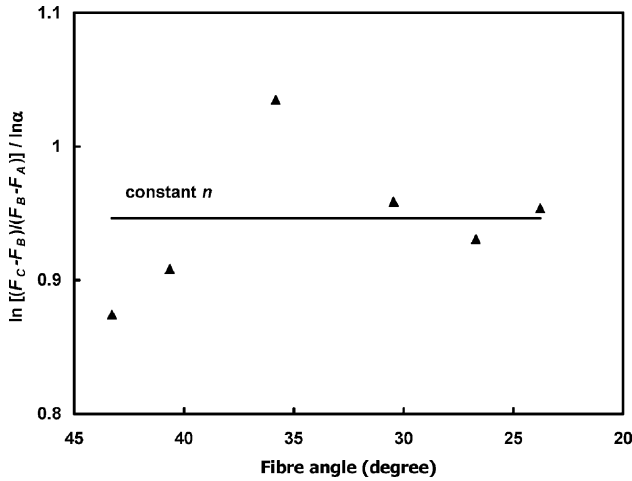
Fig. 4. Determination of power law viscosity index from experimental data.
