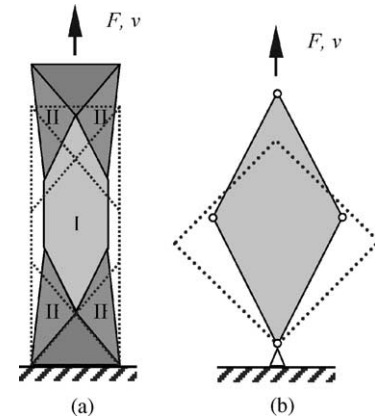
Fig. 3. Deformation profiles of woven fabric under (a) bias tension; (b) picture frame test. At initial state (shown by dotted line), the fibres are along \pm 45^\circ against the loading direction.
