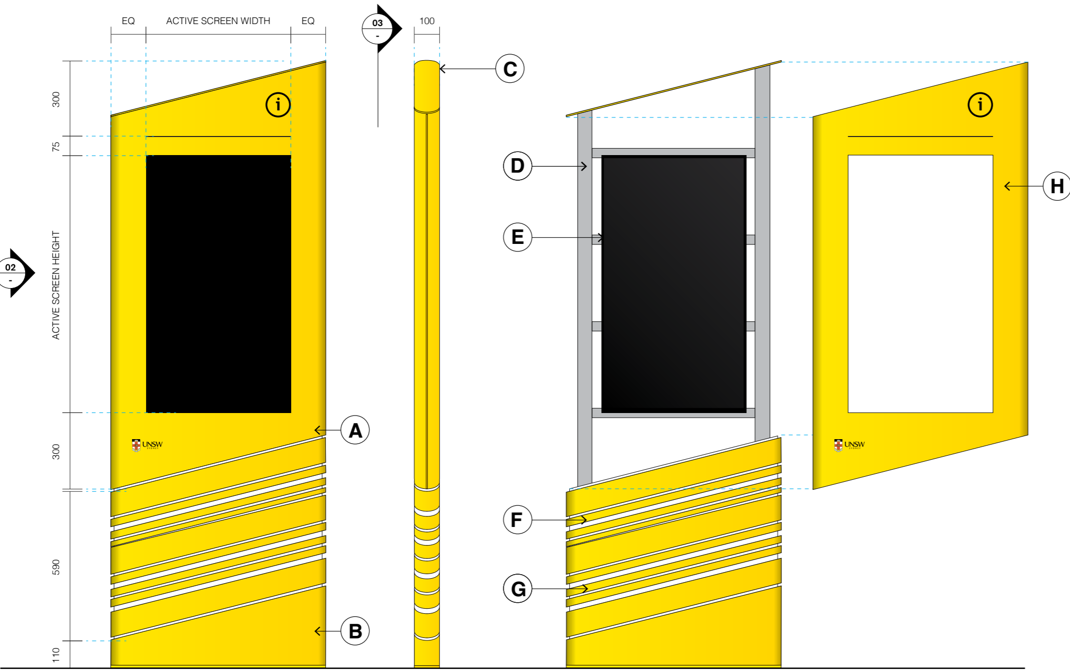
01 Front Elevation Scale 1:15
