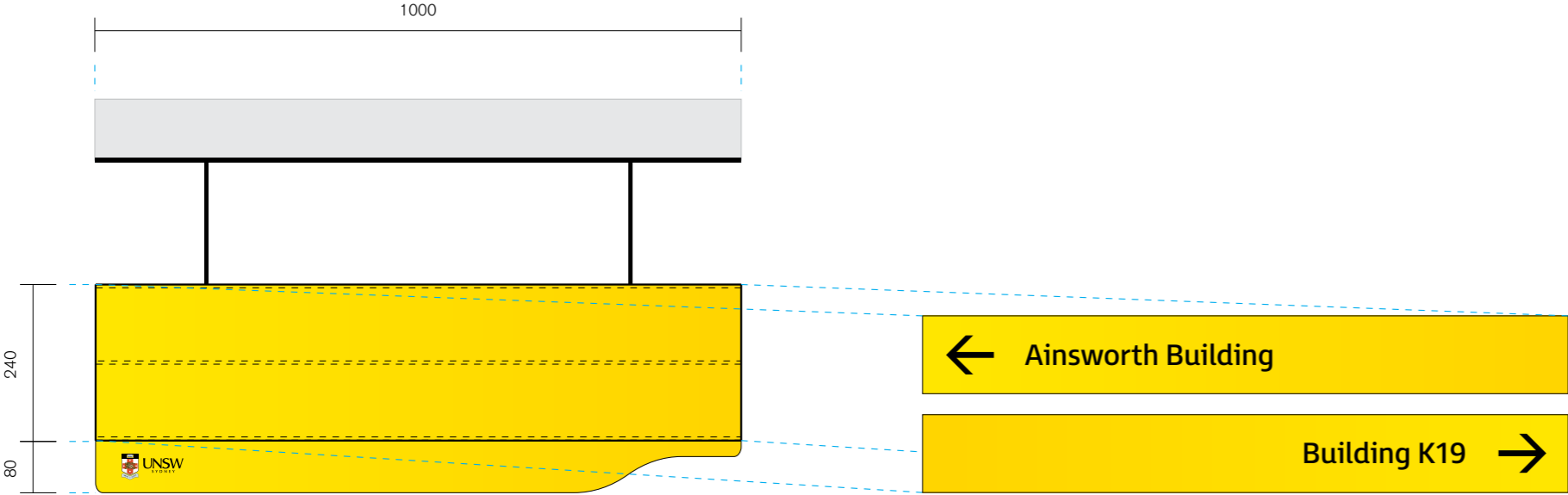
01 Elevation - Two panels Scale 1:10
