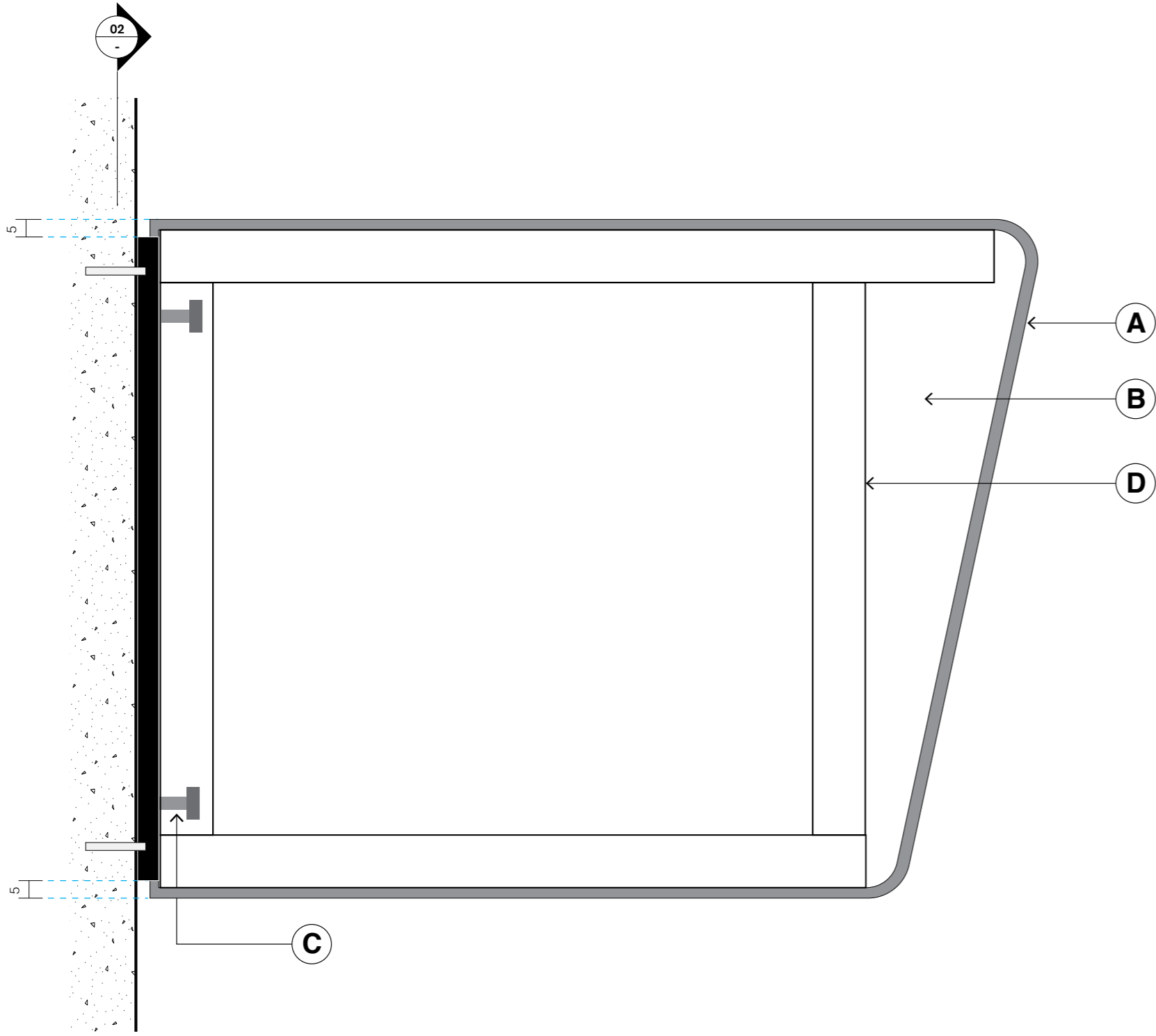
01 Section Scale 1:2
