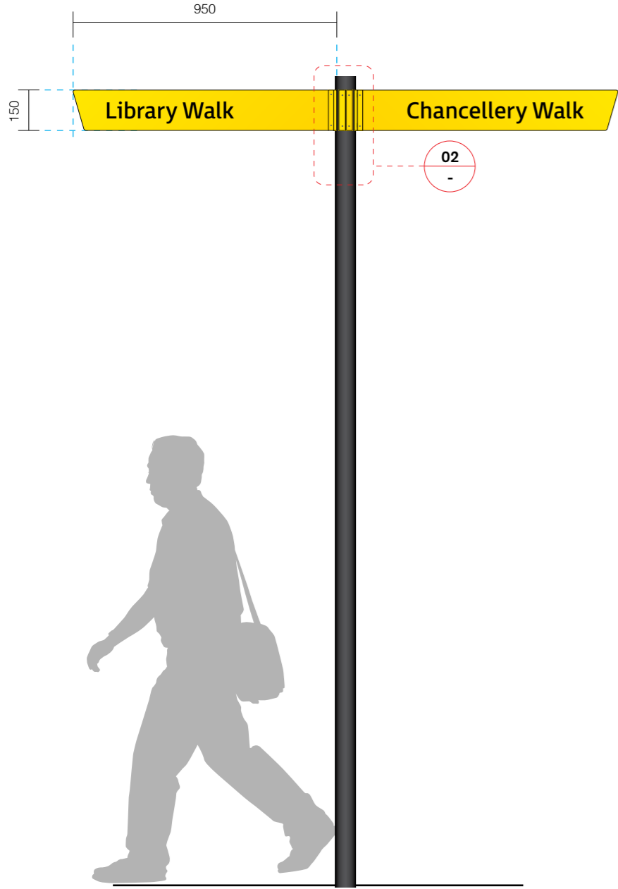
01 Elevation Scale 1:20
