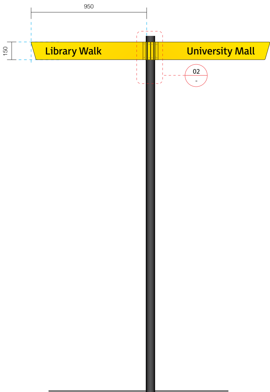
01 Elevation Scale 1:20
