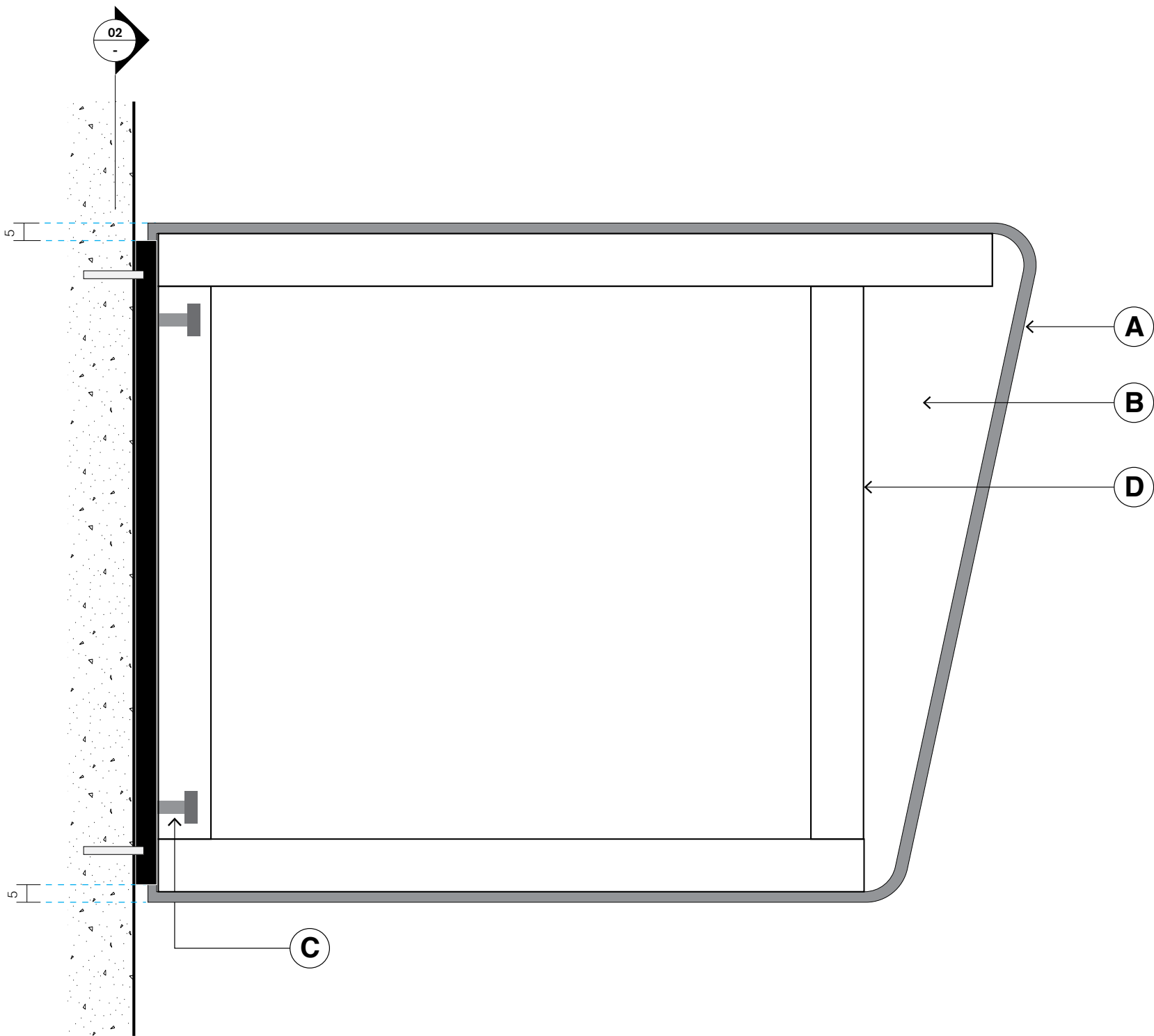
01 Section Scale 1:2
