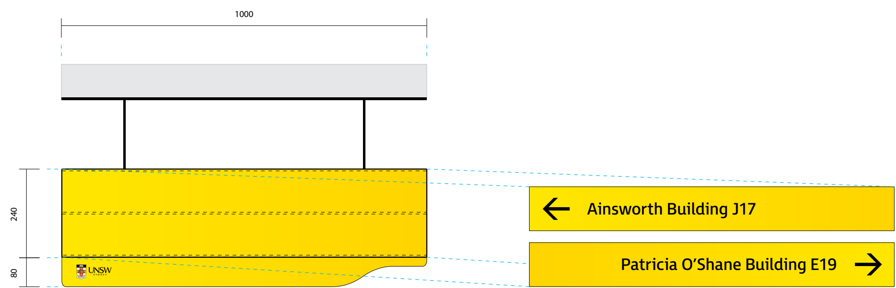
01 Elevation - Two panels Scale 1:10
