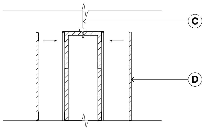
03 Detail Scale 1:1
