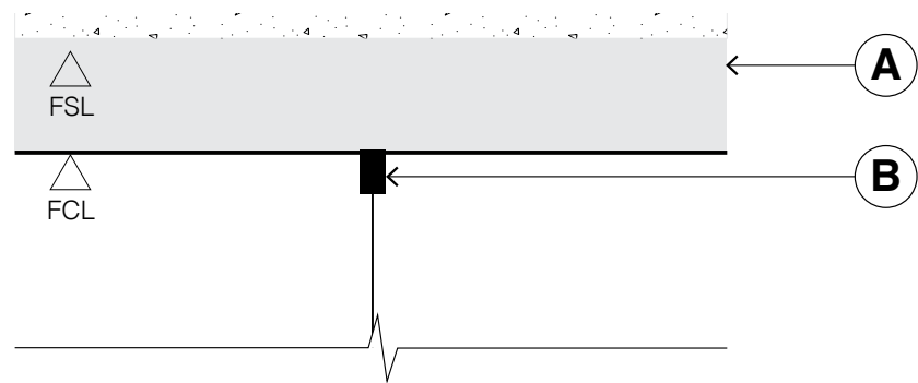
02 Detail Scale 1:1
