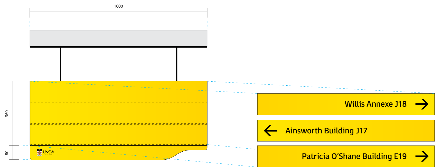
02 Elevation - Three panels Scale 1:10
