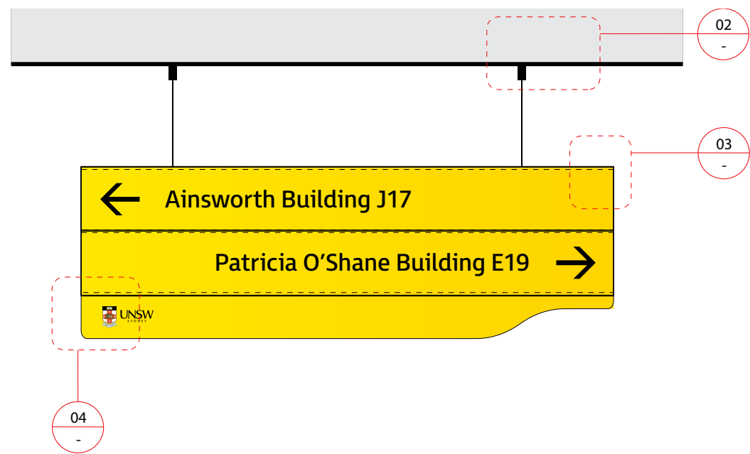
01 Elevation Scale 1:10
