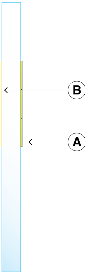
02 Elevation Glazing-mounted Scale 1:5
