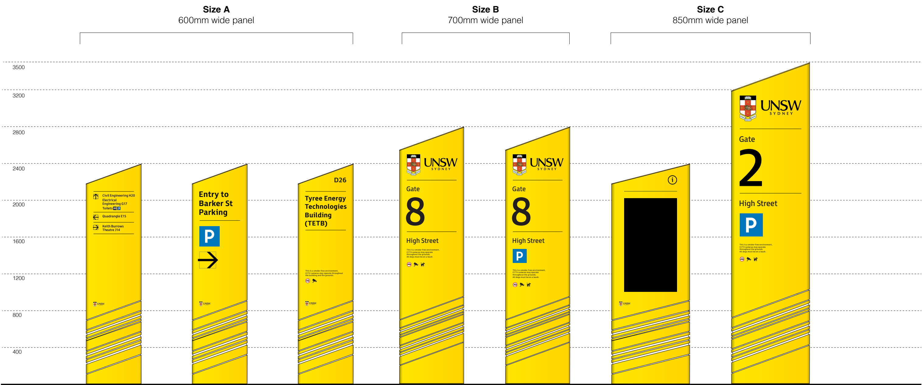
Totem heights Scale 1:25
