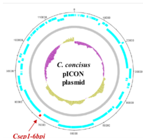
Circularised diagram of the pCON plasmid in C. concisus strain P2CDO4.
