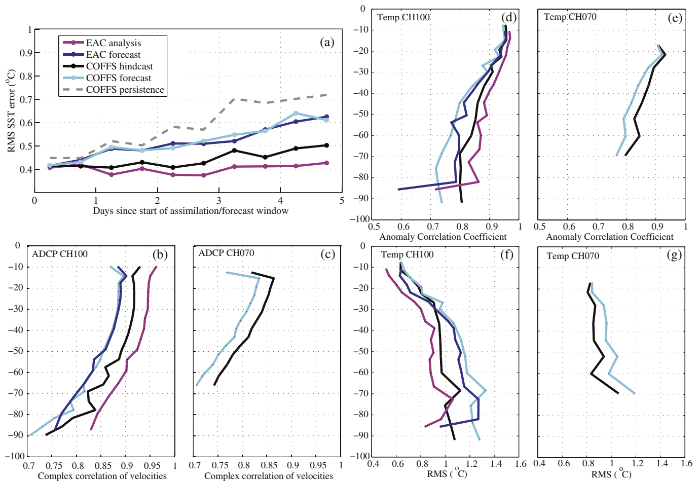
Fig. 5. Root-Mean-Squared SST error for days 0–5 of the assimilation/forecast windows, spatially-averaged over the COFFS model domain and averaged over all windows, (a). Complex correlation of velocities measured by ADCPs at CH100 (b) and CH070 (c). Anomaly Correlation Coefficient of temperature measured at CH100 (d) and CH070 (e). Root-Mean-Squared error of temperature measured at CH100 (f) and CH070 (g).
