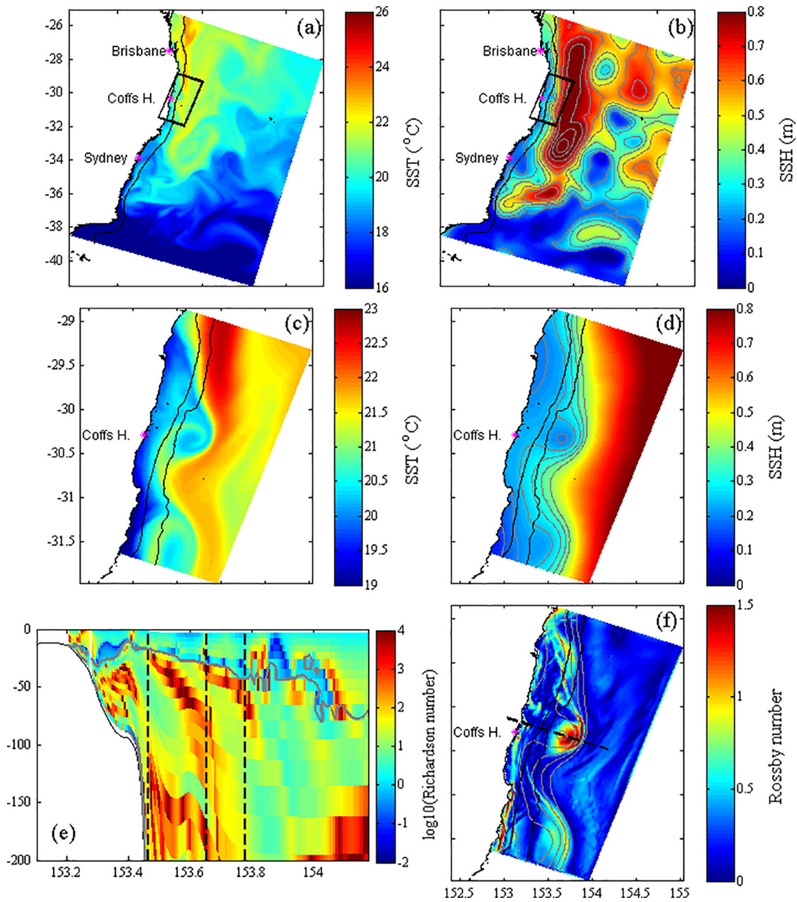
Fig. 16. Instantaneous SST, SSH, Ri and Ro numbers on 29 July 2013 from the models. SST (a) and SSH (b) from the EAC analysis and SST (c) and SSH (d) from the COFFS hindcast. The 1000 m model bathymetry contour is shown for the EAC domain (a and b, black line) and SSH contours are every 0.1 m (grey lines). For the COFFS domain (c and d), the 100 m and 1000 m model bathymetry contours are shown (black lines) and the SSH contours are every 0.05 m (grey lines). Note that the SSH magnitudes differ for the EAC and COFFS domain as COFFS includes the tides. Ri number for the COFFS hindcast (e) through the section shown by the black dashed line in (f). The vertical black dashed lines show the inshore, centre, and offshore extent of the eddy, and the grey line depicts Ri = 1. Ro number for the COFFS hindcast (f).
