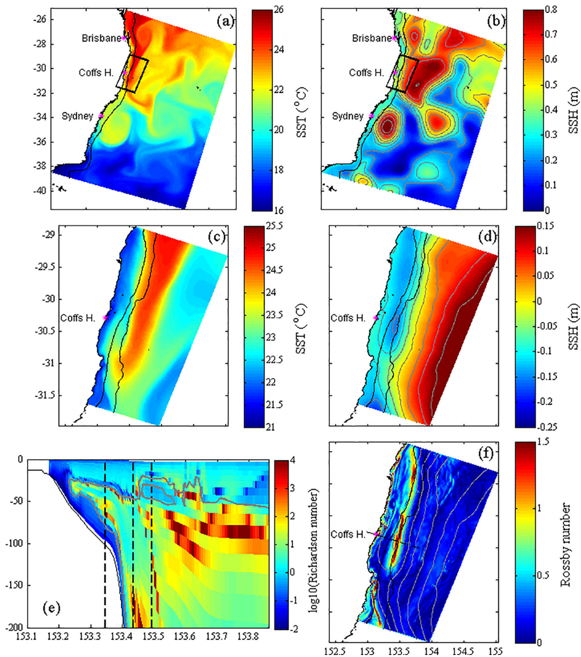
Fig. 14. Instantaneous SST, SSH, Ri and Ro numbers on 15 May 2012 from the models. SST (a) and SSH (b) from the EAC analysis and SST (c) and SSH (d) from the COFFS hindcast. The 1000 m model bathymetry contour is shown for the EAC domain (a and b, black line) and SSH contours are every 0.1 m (grey lines). For the COFFS domain (c and d), the 100 m and 1000 m model bathymetry contours are shown (black lines) and the SSH contours are every 0.05 m (grey lines). Note that the SSH magnitudes differ for the EAC and COFFS domain as COFFS includes the tides. Ri number for the COFFS hindcast (e) through the section shown by the black dashed line in (f). The vertical black dashed lines show the inshore, centre, and offshore extent of the eddy, and the grey line depicts Ri = 1. Ro number for the COFFS hindcast (f).
