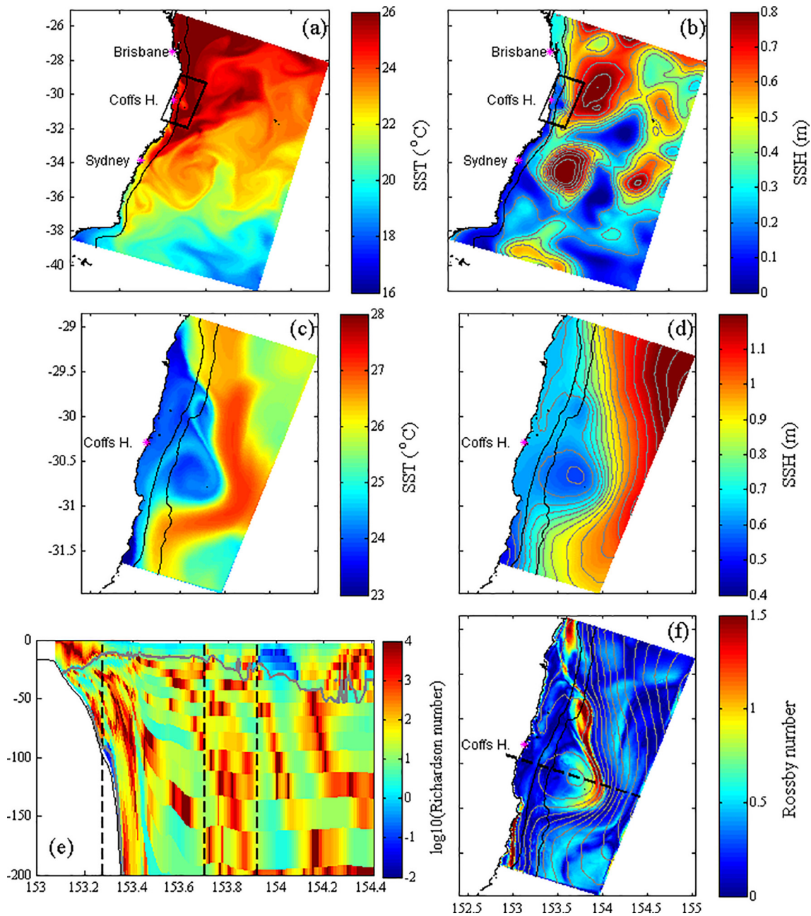
Fig. 12. Instantaneous SST, SSH, Ri and Ro numbers on 21 March 2012 from the models. SST (a) and SSH (b) from the EAC analysis and SST (c) and SSH (d) from the COFFS hindcast. The 1000 m model bathymetry contour is shown for the EAC domain (a and b, black line) and SSH contours are every 0.1 m (grey lines). For the COFFS domain (c and d), the 100 m and 1000 m model bathymetry contours are shown (black lines) and the SSH contours are every 0.05 m (grey lines). Note that the SSH magnitudes differ for the EAC and COFFS domain as COFFS includes the tides. Ri number for the COFFS hindcast (e) through the section shown by the black dashed line in (f). The vertical black dashed lines show the inshore, centre, and offshore extent of the eddy, and the grey line depicts Ri = 1. Ro number for the COFFS hindcast (f).
