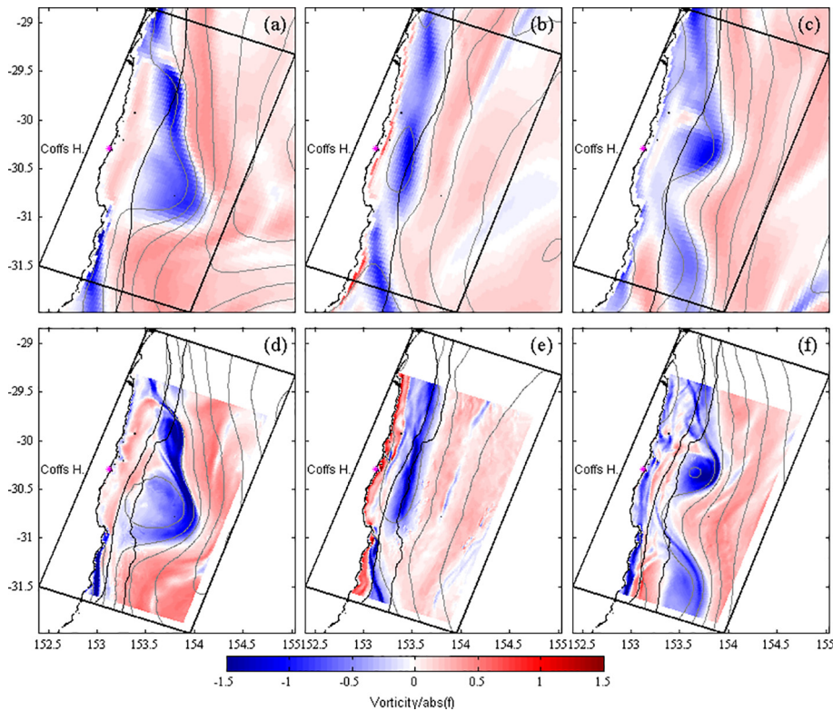
Fig. 11. Relative surface vorticity ( \zeta/|f| ) snapshots for 21 Mar 12 (EACmodel, a, and COFFS model, d), 15 May 12 (EACmodel, b, and COFFS model, e), and 29 Jul 13 (EACmodel, c, and COFFS model, f). The bold black box shows the boundaries of the COFFS model domain. The 1000 m model bathymetry contour is shown for the EAC model (a–c, black lines) and the 100 m and 1000 m model bathymetry contours are shown for the COFFS model (d–f, black lines). SSH contours are every 0.1 m (grey lines). Note that the SSH magnitudes differ for the EAC and COFFS domain as COFFS includes the tides. The plots of the COFFS domain (d–f) exclude 10 grid cells inside of the eastern and southern boundaries (the sponge layer) and 60 grid cells from the northern boundary (the sponge layer is 30 grid cells wide here but 60 grid cells are required for the bathymetric merging between the EAC model and the COFFS model).
