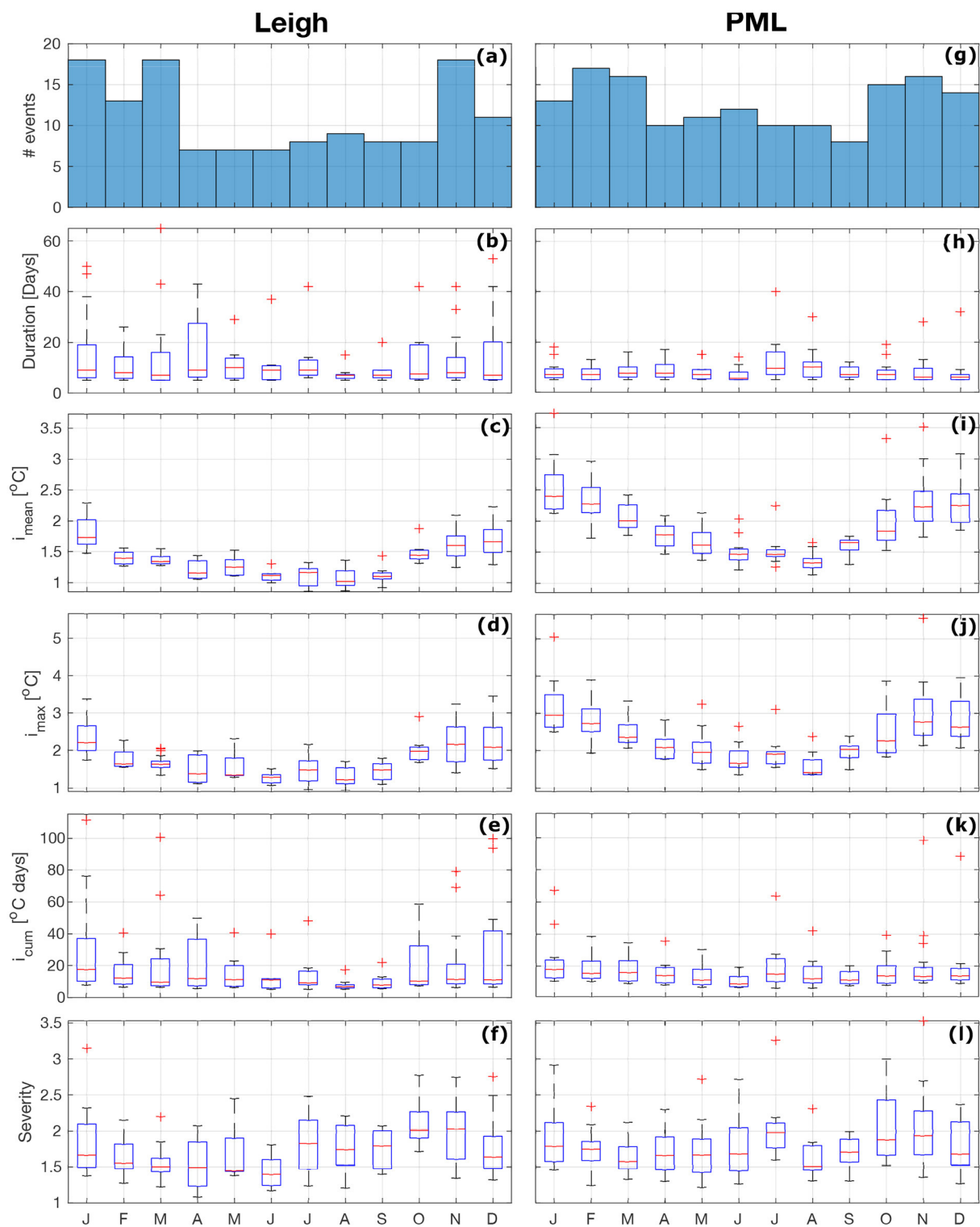
FIGURE 4 MHW metrics from detected events at Leigh (a–f) and PML (g–l) sorted by month. (a,g) Are histograms of event numbers for each month with box plots (b–f,h–l) of event duration, intensities (mean, maximum, and cumulative) and severity also displayed. Seasonality in mean (c,i) and maximum (d,j) intensity is observed but no clear patterns are observed for duration (b,h), cumulative intensity (e,k), and severity (f,l).
