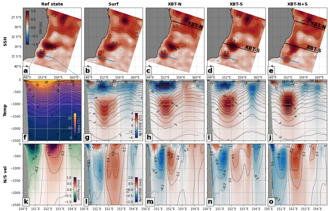
Figure 7. The vertical representation of an anticyclonic–cyclonic eddy pair at \sim 37.5^\circ S, 151.5 – 153.5^\circ E in the (a) Ref state is compared to the (b) Surf, (c) XBT-N, (d) XBT-S, and (e) XBT-N+S OSSEs, with the SSH field and vertical profile location marked by a blue line. The vertical temperature profile along the transect is shown for the (f) Ref state and the (g) Surf, (h) XBT-N, (i) XBT-S, and (j) XBT-N+S OSSEs. Likewise, (k–o) northward velocity profiles are shown for the same experiments. In the OSSE panels, the difference in temperature and velocity from the Ref state plotted in colour and contours of (dark colour) the OSSE and (light colour) the respective field in the Ref state are shown for comparison. In panel (a), the blue dashed lines indicate the transect shown in (f). The XBT-N and XBT-S transect locations are marked in the respective panels. Axes with latitudes are labelled ^\circ S, and axes with longitudes are labelled ^\circ E.
