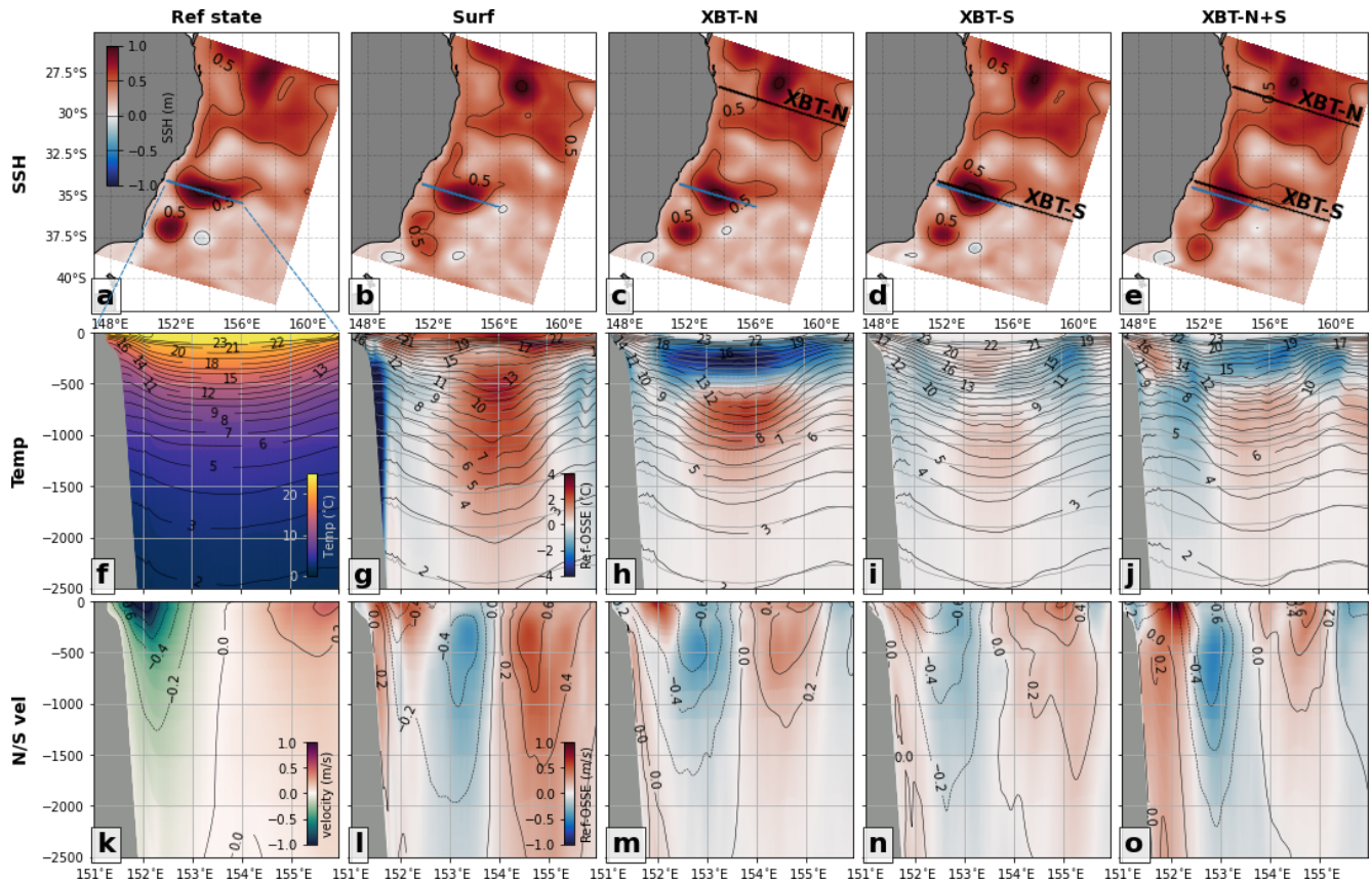
Figure 6. The vertical representation of an anticyclonic eddy at \sim 35^\circ S, 153^\circ E in the (a) Ref state is compared to the (b) Surf, (c) XBT-N, (d) XBT-S, and (e) XBT-N+S OSSEs, with the SSH field and vertical profile location marked by a blue line. The vertical temperature profile along the transect is shown for the (f) Ref state and the (g) Surf, (h) XBT-N, (i) XBT-S, and (j) XBT-N+S OSSEs. Likewise, (k–o) northward velocity profiles are shown for the same experiments. In the OSSE panels, the difference in temperature and velocity from the Ref state plotted in colour and contours of (dark colour) the OSSE and (light colour) the respective field in the Ref state are shown for comparison. In panel (a), the blue dashed lines indicate the transect shown in (f). The XBT-N and XBT-S transect locations are marked in the respective panels. Axes with latitudes are labelled ^\circ S, and axes with longitudes are labelled ^\circ E.
