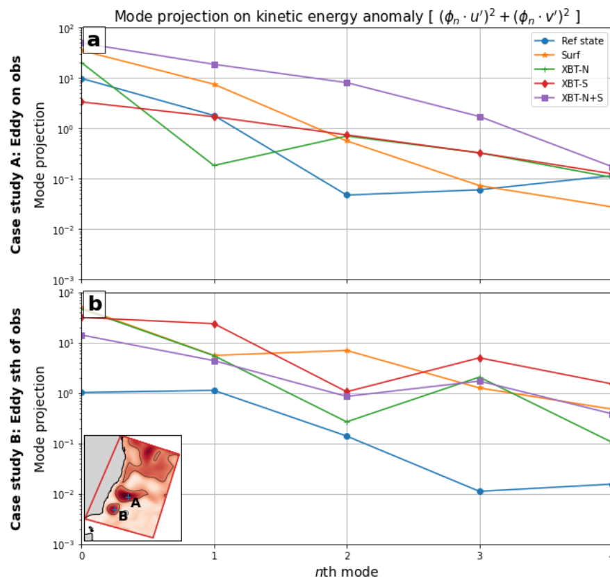
Figure 10. The barotropic and baroclinic modes are projected onto the kinetic energy through the squared addition of the mode projections on the zonal and meridional velocity anomalies (see Sect. 2.3.4). In (a), the value of the n th mode projections for case study A are shown, and in (b), the n th mode projections for case study B are shown. The locations of case studies A and B are shown in the inset in (b).
