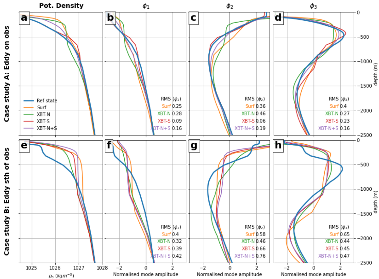
Figure 9. For case study A, the (a) potential density profile is shown for the Ref state and each OSSE, and the amplitude of the baroclinic modes (b) \phi_1 , (c) \phi_2 , and (d) \phi_3 are shown for the Ref state and each OSSE. For case study B, the (e) potential density profile and baroclinic modes (f) \phi_1 , (g) \phi_2 , and (h) \phi_3 are shown for the Ref state and each OSSE. The barotropic mode ( \phi_0 ) is excluded, as by normalisation it has unity value at all depths. Potential densities are referenced to surface pressure. In panels (b)–(d) and (f)–(h), we show the rms difference of the OSSE mode shape compared to that of the Ref state. Note that the vertical axis has been limited to the top 2500 m.
