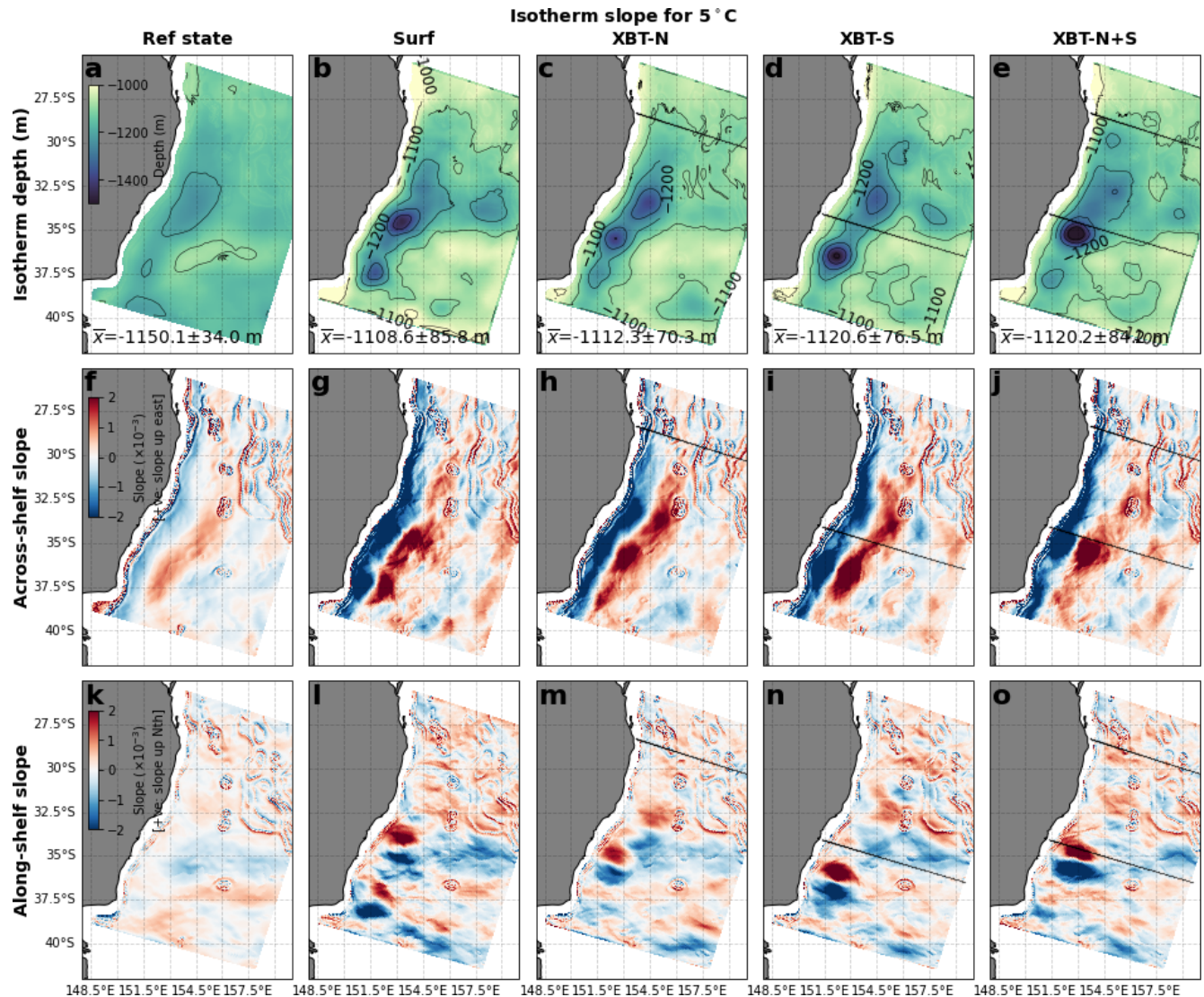
Figure 5. The depth of the 5 °C isotherm is shown for (a) the Ref state and the (b) Surf, (c) XBT-N (d) XBT-S, and (e) XBT-N+S OSSEs. The across-shelf isotherm slope at the 5 °C isotherm is shown for the (f) Ref state and the (g) Surf, (h) XBT-N, (i) XBT-S, and (j) XBT-N+S OSSEs. Likewise, the along-shelf slope of the 5 °C isotherm is shown for the (k) Ref state and the (l) Surf, (m) XBT-N, (n) XBT-S, and (o) XBT-N+S OSSEs. A positive across-shelf slope is upwards sloping towards the east, and a positive along-shelf slope is upwards sloping towards the north. The XBT-N and XBT-S transect locations are marked in the respective panels. Axes with latitudes are labelled ° S, and axes with longitudes are labelled ° E.
