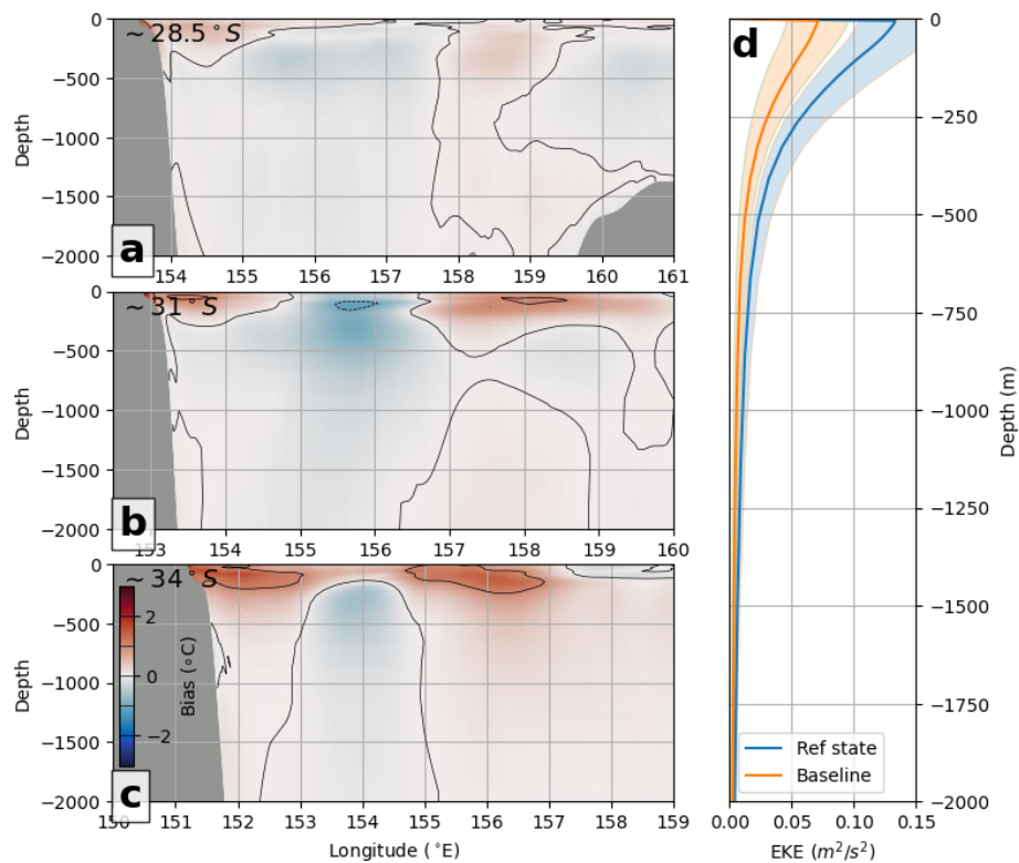
Figure A1. The temperature bias between the baseline and the Ref state is shown at three transects, (a) \sim 28.5^\circ S, (b) \sim 31^\circ S, and (c) \sim 34^\circ S. In (d), the depth profile of EKE, averaged over the high-EKE box (see box in Fig. 3a), for the Ref state and baseline experiments.
