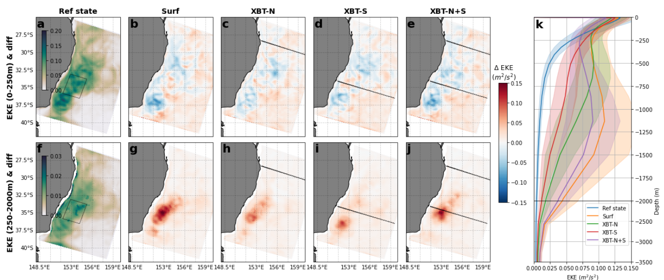
Figure 3. The time-mean eddy kinetic energy (EKE) is shown as the average over the top 250 m for (a) the Ref state, and the difference from this for the (b) Surf, (c) XBT-N (d) XBT-S, and (e) XBT-N+S OSSEs and as the average over 250–2000 m for (f) the Ref state and the difference from this for the (g) Surf, (h) XBT-N (i) XBT-S, and (j) XBT-N+S OSSEs. In (k), the vertical profile of the EKE, spatially averaged over the high eddy variability region (box shown in panels a and f), is shown for each OSSE. The shaded regions designate a range of plus and minus 1 standard deviation in spatial mean EKE at that depth for that OSSE. The XBT-N and XBT-S transect locations are marked in the respective panels. Axes with latitudes are labelled ^{\circ}\text{S} , and axes with longitudes are labelled ^{\circ}\text{E} .
