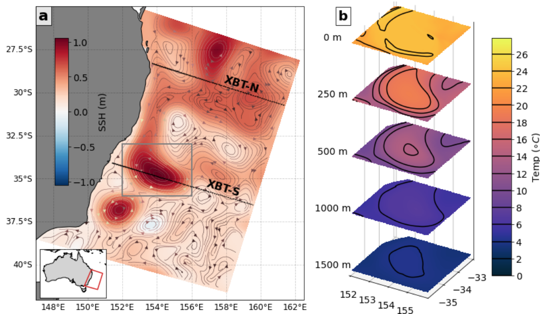
Figure 1. (a) The East Australian Current region is shown, with lines of subsurface observations marked in the north (XBT-N) and south (XBT-S) of the domain (black lines). The colour map shows the mean model sea surface height (SSH) during the 6–12 March 2012, with streamlines calculated from surface velocities marked as vectors. The study region is shown as an inset on the east coast of Australia. The grey box shows the region in focus in panel (b), which shows the vertical structure of temperature at various levels (0, 250, 500, 1000, and 1500 m) for a region focussing on an anticyclonic (warm core) eddy. Black contours of temperature are shown in (b), with intervals marked in the colour bar.
