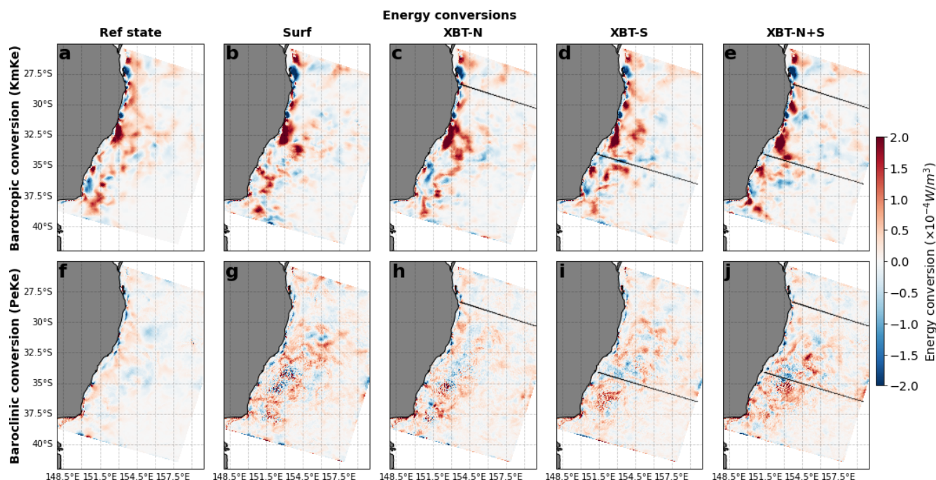
Figure 8. The barotropic conversion rate (KmKe) is shown for the (a) Ref state and (b) Surf, (c) XBT-N, (d) XBT-S, and (e) XBT-N+S OSSEs. The baroclinic conversion rate (PeKe) is shown for the (f) Ref state and (g) Surf, (h) XBT-N, (i) XBT-S, and (j) XBT-N+S OSSEs. In all panels, a positive value indicates conversion from (for panels a–e) mean kinetic or (for panels f–j) eddy potential energy into eddy kinetic energy. The XBT-N and XBT-S transect locations are marked in the respective panels. Axes with latitudes are labelled ° S, and axes with longitudes are labelled ° E.
