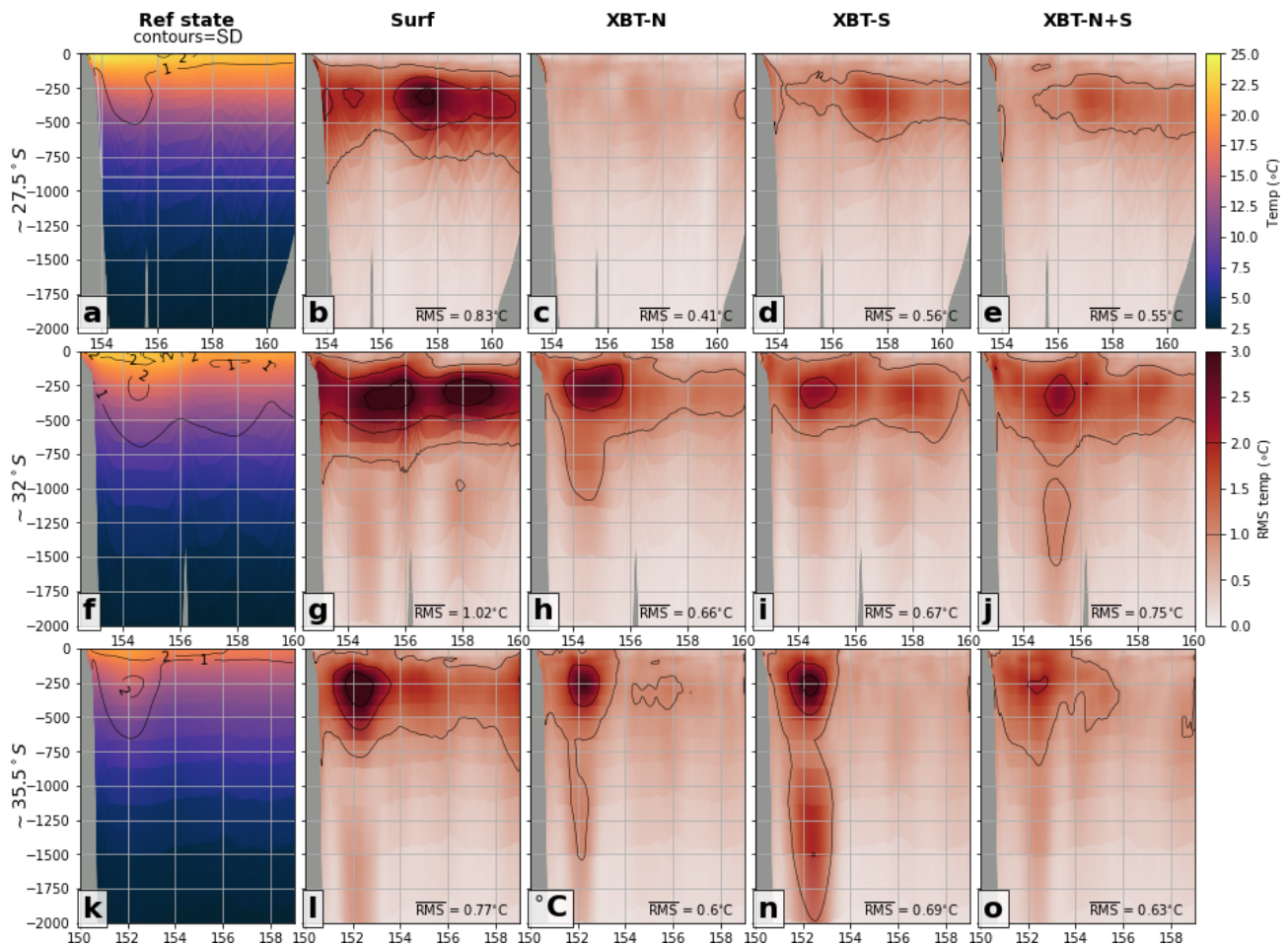
Figure 7. Differences in vertical transects of temperature for each experiment are shown for the \sim 27.5^\circ , \sim 32^\circ , and \sim 35.5^\circ S transects. (a) The mean temperature of the reference state with contours of standard deviation. The rms error between the reference state and the OSSEs (b) surf, (c) XBT-N, (d) XBT-S, and (e) XBT-N+S is shown at the \sim 27.5^\circ S transect. The second row (f–j) shows the same fields as the first row, but for the second transect at \sim 32^\circ S, while the third row (k–o) shows the same fields but for the third transect at \sim 35.5^\circ S. In reference state panels, contours are the standard deviation in the respective field while in all OSSE panels, the contours are of RMSE. Contour intervals are shown as a line in the RMSE colour bar. The depth-averaged RMSE of the region shown in each panel is included in the bottom corner.
