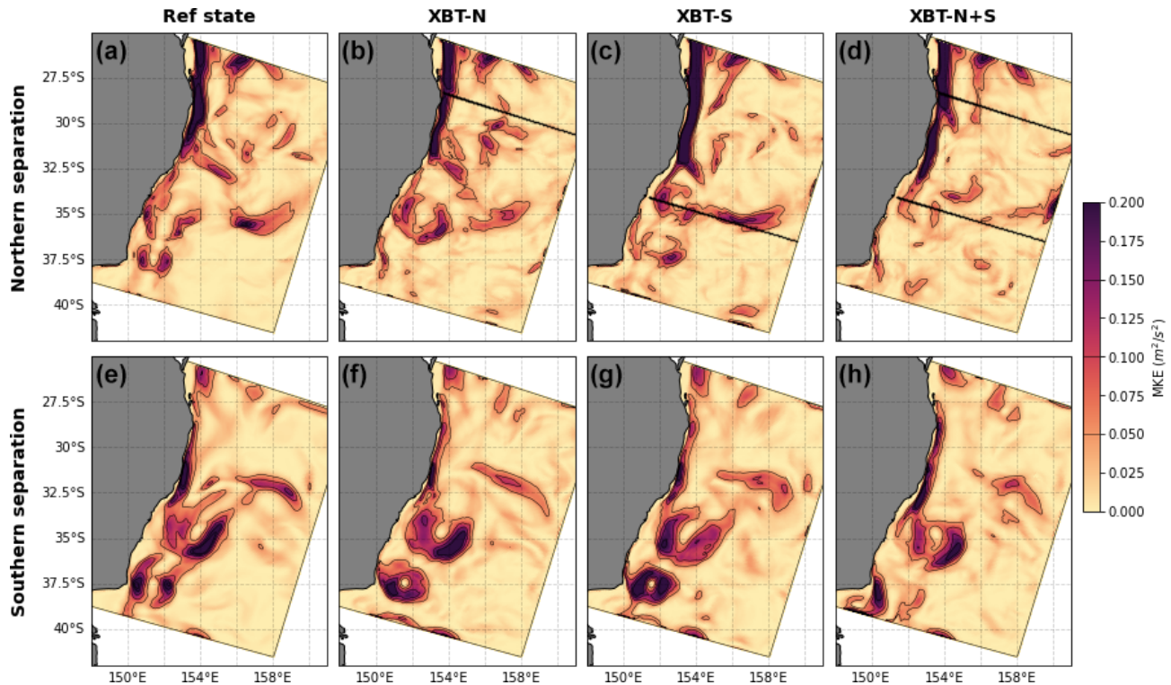
Figure 9. The surface MKE is compared between the (a) reference state, (b) XBT-N, (c) XBT-S, and (d) XBT-N+S for the case when the EAC is in a northern separation phase. For the southern separating EAC phase, the surface MKE is compared between the (e) reference state and the (f) XBT-N, (g) XBT-S, and (h) XBT-N+S. Black lines in panels (b–d) indicate location of the XBT lines.
