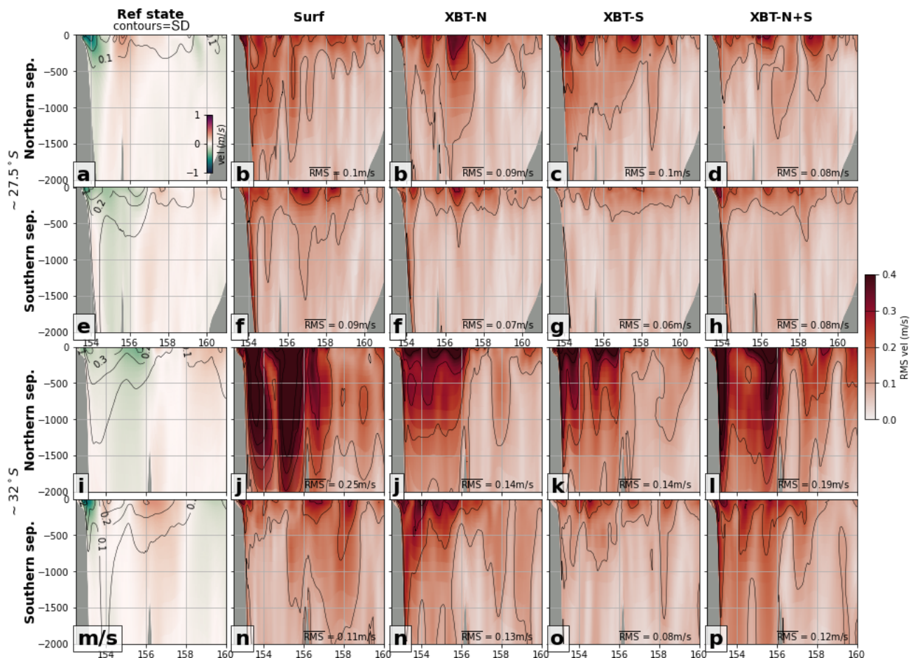
Figure 10. The northwards velocity at \sim 27.5^\circ\text{S} is compared between the (a) reference state, (b) XBT-N, (c) XBT-S, and (d) XBT-N+S for the case when the EAC is in a northern separation phase, and for the (e) reference state, (f) XBT-N, (g) XBT-S, and (h) XBT-N+S in the southern separation phase. Likewise, the northward velocity is compared along the transect at \sim 32^\circ\text{S} for the (i) reference state, (j) XBT-N, (k) XBT-S, and (l) XBT-N+S OSSEs in the case when the EAC is in a northern separation phase. Lastly, velocities along the same transect in the (m) reference state, (n) XBT-N, (o) XBT-S, and (p) XBT-N+S OSSEs are compared for the southern separation phase. In the reference state panels, contours are the standard deviation in the respective field while in all OSSE panels, the contours are of RMSE. Contour intervals are shown as a line in the RMSE colour bar. The depth-averaged RMSE of the region shown in each panel is included in the bottom corner.
