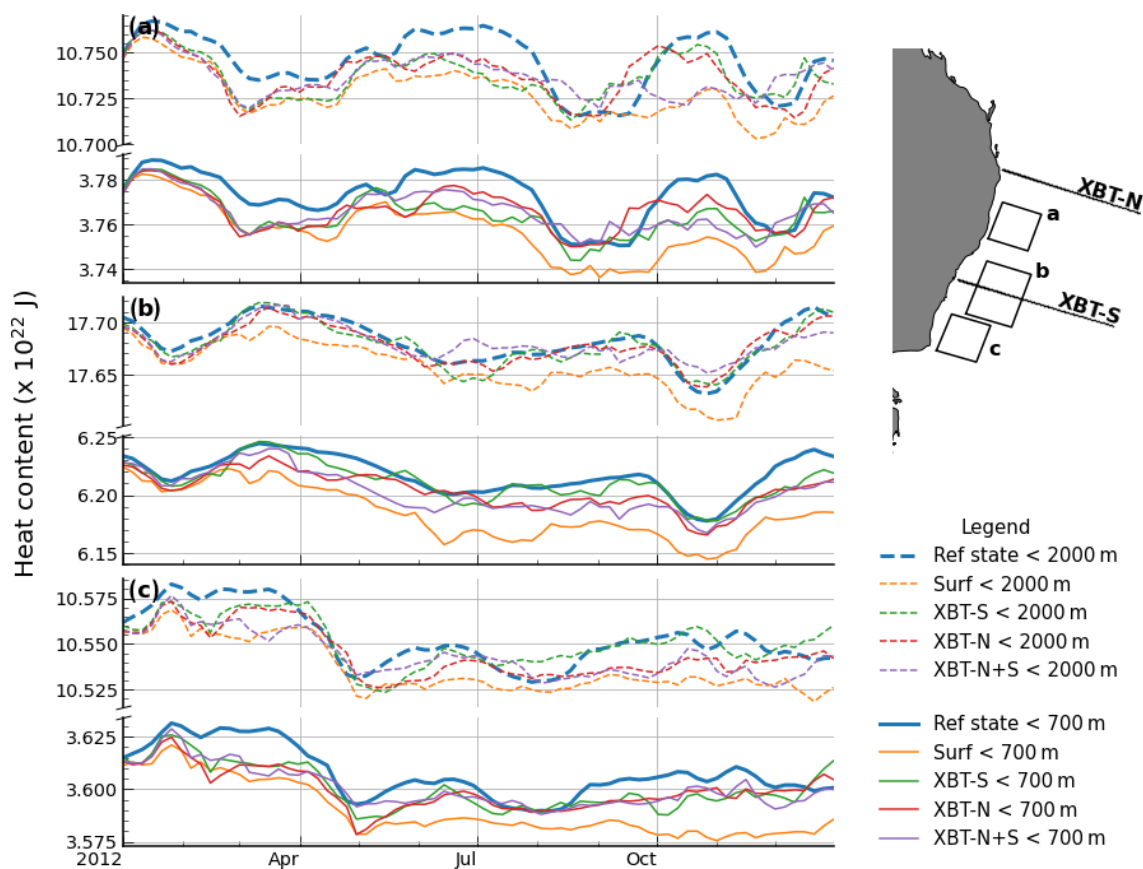
Figure 8. The temporal evolution of integrated upper ocean heat content for three key regions: (a) upstream of the EAC separation zone, (b) the high EKE variability region, and (c) the region with strong UOHC trends, with locations shown in inset. The upper 700 m is shown with solid lines and the upper 2000 m is shown with dashed lines. Note the broken y axes.
