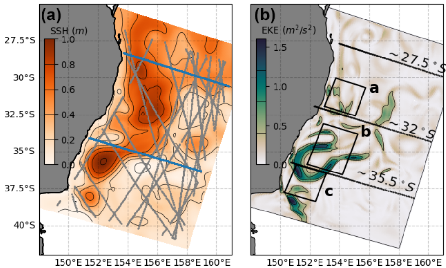
Figure 3. Snapshots of model conditions with examples of observations and analysis regions. (a) A snapshot of SSH (colour map) is shown with a single 5 d cycle of SSH (grey dots) and XBT (blue dots) observations. (b) A snapshot of EKE (colour map) is shown, with boxes and lines showing key regions and diagnostic transects used in the analysis.
