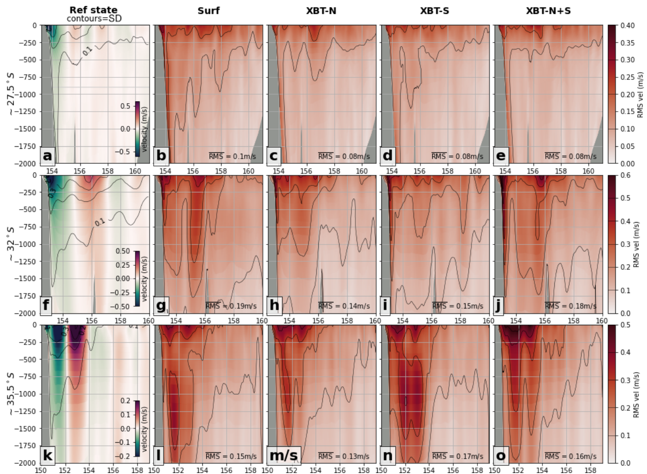
Figure 6. Vertical cross-sections of meridional (north/south) velocity at key transects (first row) \sim 27.5^\circ S, (second row) \sim 32^\circ S, and (third row) \sim 35.5^\circ S are shown for each experiment. (a) The time-mean velocity (northwards–positive) in the reference state, with contours of standard deviation in the reference state velocity. The rms error between the reference state and the OSSEs (b) surf, (c) XBT-N, (d) XBT-S, and (e) XBT-N+ is shown at the transect \sim 27.5^\circ S. The second row (f–j) shows the same fields as the first row, but for the second transect at \sim 32^\circ S, while the third row (k–o) shows the same fields but for the third transect at \sim 35.5^\circ S. In reference state panels, contours are the standard deviation in the respective field while in all OSSE panels, the contours are of RMSE. Contour intervals are shown as a line in the RMSE colour bar. The depth-averaged RMSE of the region shown in each panel is included in the bottom corner.
