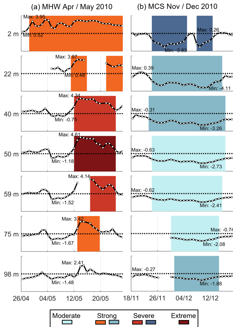
Figure 5. Examples of a MHW and MCS over depth at the PHB/PH100 site: (a) MHW in April and May 2010 and (b) MCS in November and December 2010. The daily varying temperature anomalies ( ^{\circ}\text{C} ) relative to the mean (black line with white dots) are shown for each depth. Time periods when MHWs or MCSs occur are shaded, with colours indicating the category (“Moderate”, “Strong”, “Severe” and “Extreme”) as shown in the legend. The maximum and minimum temperature anomaly relative to the mean for each time period and depth is also shown.
