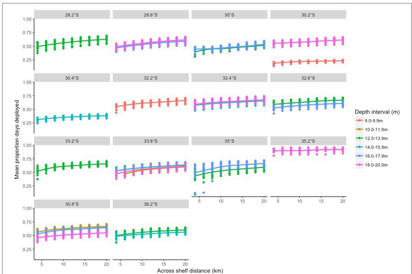
FIGURE 5 | Mean proportion of days that loggers were deployed that had corresponding satellite data for different across-shelf distances.
