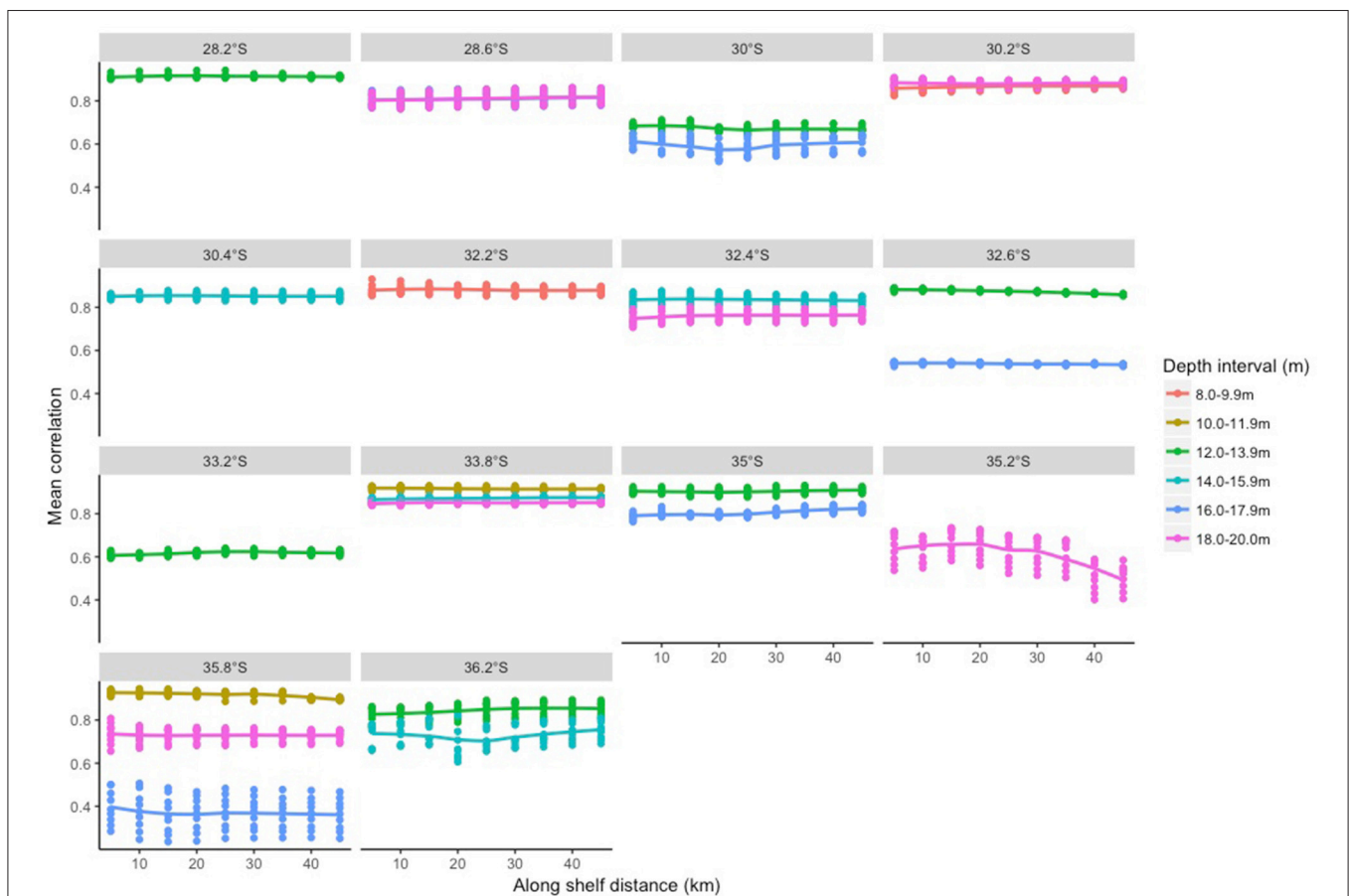
FIGURE 6 | Mean Pearson's correlation between satellite data and in situ data for different along-shelf distances.
