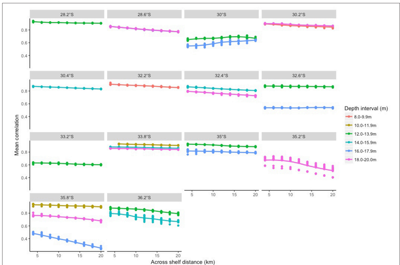
FIGURE 4 | Mean Pearson's correlation between satellite data and in situ data for different across-shelf distances.
