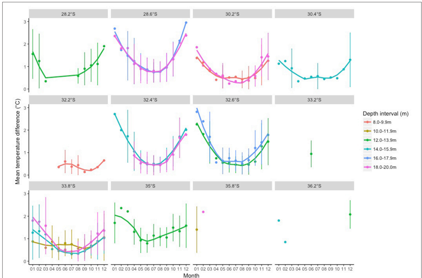
FIGURE 10 | Mean temperature differences between in situ and satellite that was processed at each logger location using an area average of 8 km across shelf and 20 km along shelf with a rolling mean based on the de-correlation time for the in situ location to fill in missing data (i.e. area- and time- averaged values).
