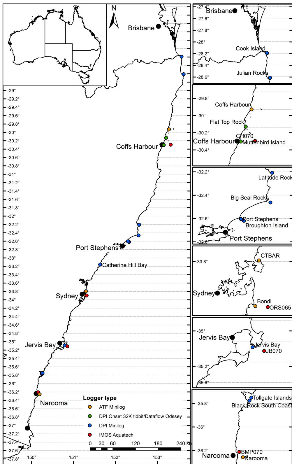
FIGURE 1 | Study site map showing the location of each in situ mooring and logger. Horizontal lines indicate the 0.20° of latitude that is used to average the data in the remaining figures.
