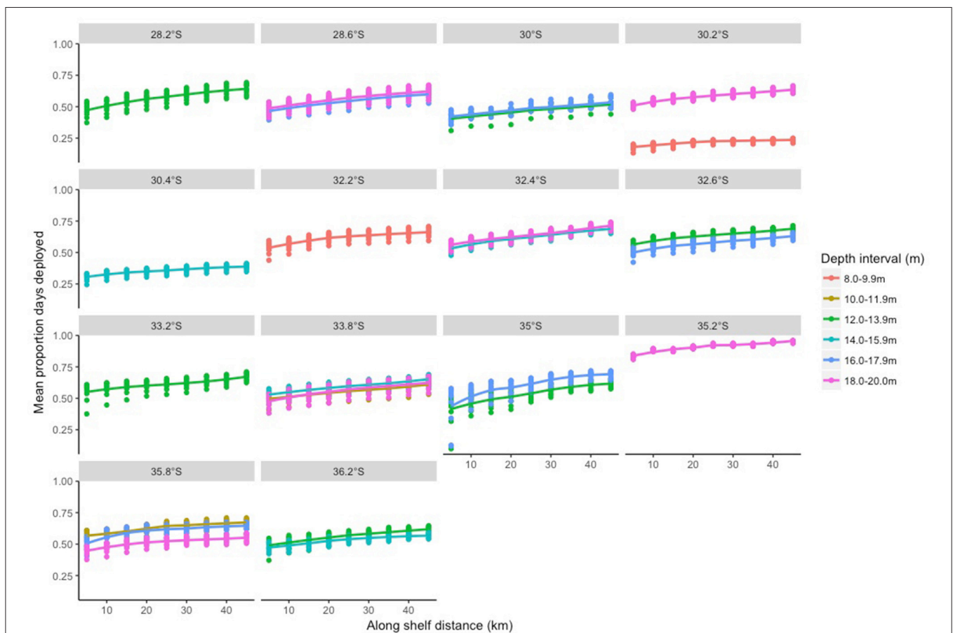
FIGURE 7 | Mean proportion of days that loggers were deployed that had corresponding satellite data for different along-shelf distances.
