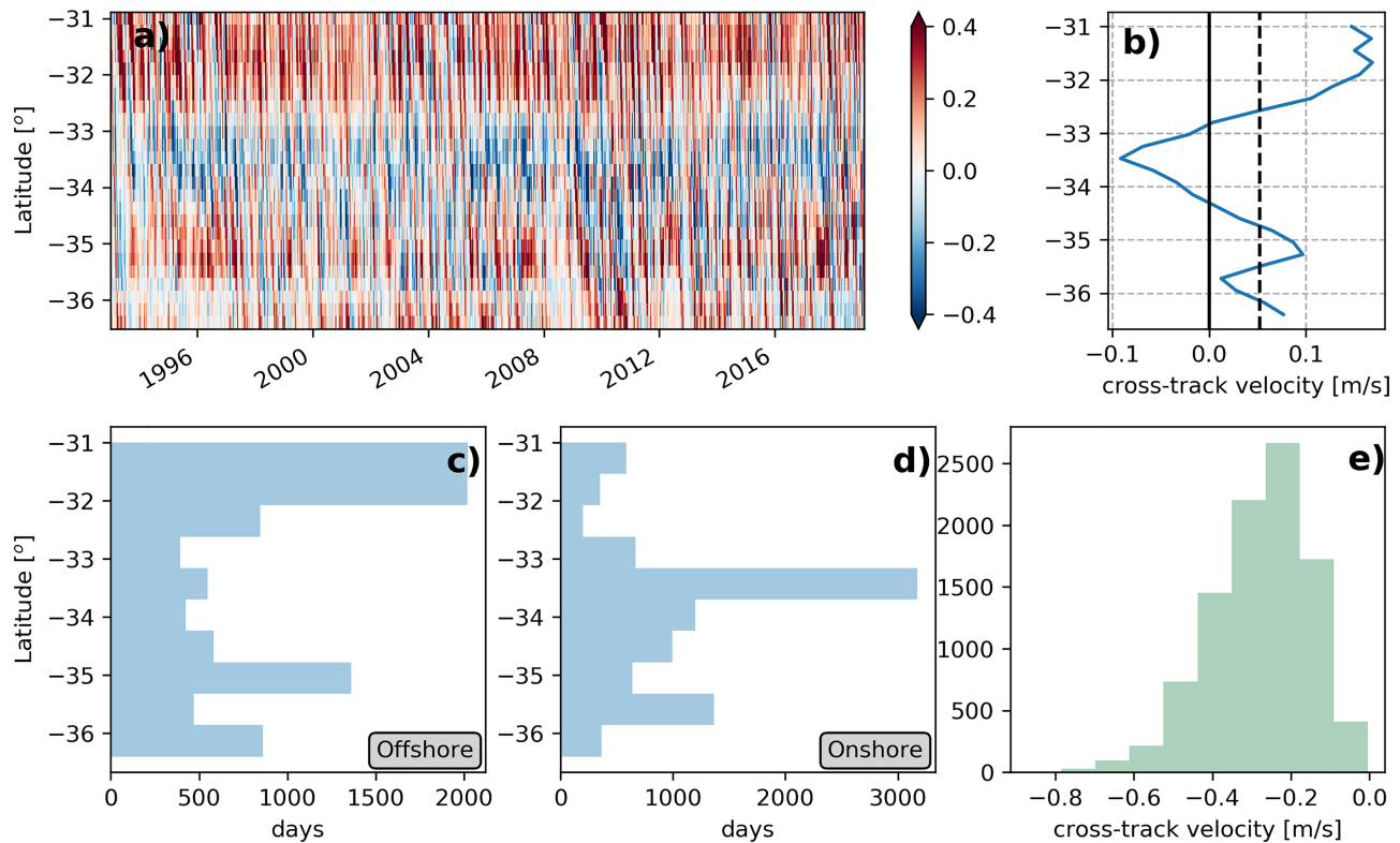
Figure 2. (a) Hovmöller plot of cross-shelf velocity along the shelf section, (b) time-mean of cross-shelf velocities from 1993–2018 (mean value shown as vertical dashed black line), (c) latitude distribution of maximum offshore velocity, (d) latitude distribution of daily maximum onshore velocity, and (e) distribution of velocity values at that maximum (negative values indicate onshore flow).
