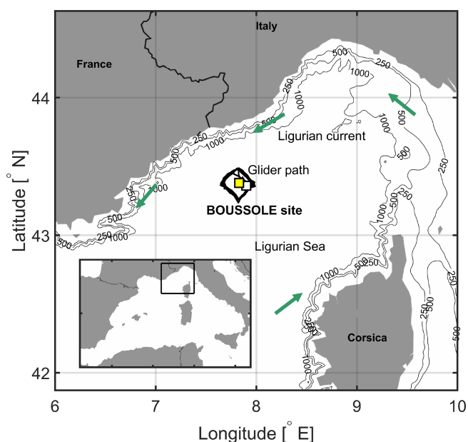
Figure 1. The area of the northwestern Mediterranean Sea showing the French Riviera and Italian Riviera, the island of Corsica, the main current branches (green arrows) in the Ligurian Sea, and the locations of the BOUSSOLE buoy (white square) and the Azur meteorological buoy (yellow square). The black line indicates the glider's path in March–April 2016.
