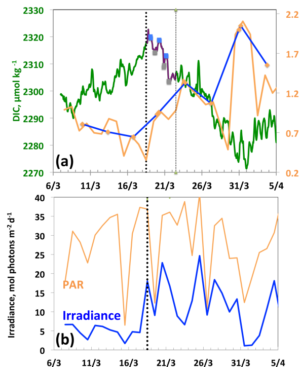
Figure 5. From 7 March to 5 April, (a) DIC and Chl a . The purple line and the squares (blue, morning; grey, evening) indicate the 3 d biological diurnal DIC changes during the period considered to compute NCP. The blue and orange lines indicate the surface Chl a when the glider was at a distance of less than 5 km (blue) and less than 20 km (orange), respectively, from the BOUSSEULE buoy. (b) PAR and I , average mixing-layer irradiance. The vertical dotted black line indicates the onset of the bloom on 18 March.
