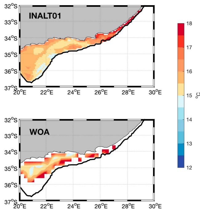
Figure 1. Depth-averaged mean temperature (°C) calculated from 1948 to 2007 for areas <200 m in depth on the central and eastern Agulhas Bank from INALT01 (top) and World Ocean Atlas observations (bottom); the black solid line shows the 200-m isobath.
