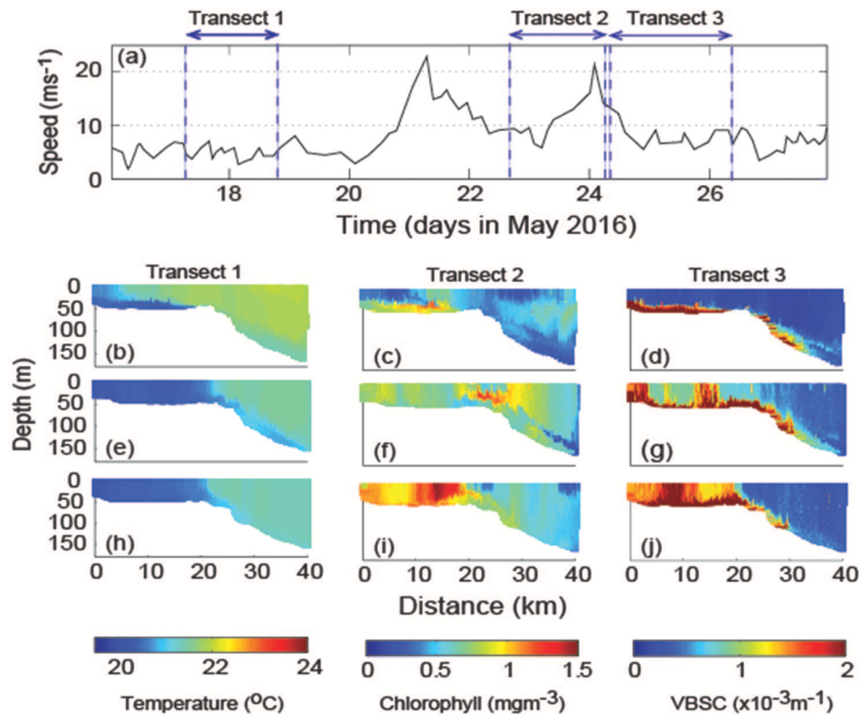
FIGURE 9 | (a) Wind speed and direction at Rottnest Island, south-west Australia. The vertical dashed lines represent timing of the ocean glider transects; Ocean glider vertical cross-sections of: (b,e,h) temperature ( ^{\circ}\text{C} ); (c,f,i) chlorophyll ( \text{mg}\cdot\text{m}^{-3} ); and, (d,g,j) backscatter ( \times 10^{-3}\text{m}^{-1} ) across the Rottnest continental shelf. The time series of wind indicate calm winds (speeds \sim 5\text{ m}\cdot\text{s}^{-1} ) followed by two winter storms (speeds > 20\text{ m}\cdot\text{s}^{-1} ). The wind speeds reduced to \sim 7\text{ m}\cdot\text{s}^{-1} on 23 May before increasing again to > 20\text{ m}\cdot\text{s}^{-1} . There were 3 cross-shore ocean glider transects during this period. During the calm period (17–18 May 2016), a well-mixed water column with cooler ( \sim 20^{\circ}\text{C} ) water was present on the inner-shelf region to 5 km from the coast. Seaward of 5 km, a dense shelf water cascade (DSWC, Pattiaratchi et al., 2011) was present and extended along the sea bed to the shelf break. On the inner shelf, chlorophyll concentrations and backscatter values were higher within the DSWC and low in the surface layer. The two storms vertically mixed the continental shelf resulting in a well-mixed water column, increased suspended sediment elevated chlorophyll concentrations (modified from Chen et al., in review).
