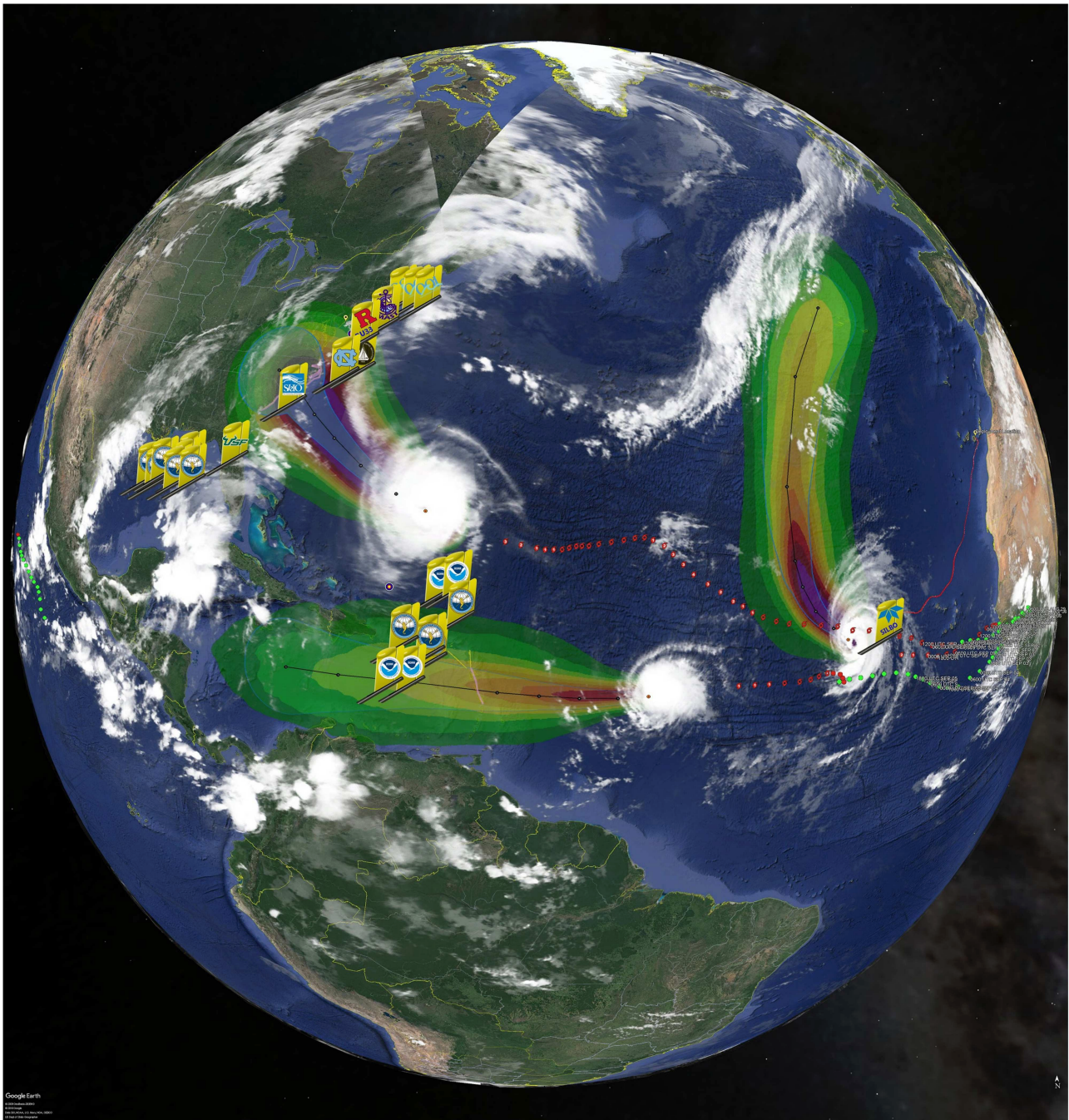
FIGURE 8 | Hurricane Florence, Isaac and Helene cloudtops (left to right) on September 11, 2018, with NHC best tracks behind each hurricane, NHC probability of tropical storm force winds ahead of each hurricane, and the tails of the diverse fleet of ocean glider in the picket lines transmitting upper ocean data in near-real time to forecasters.
