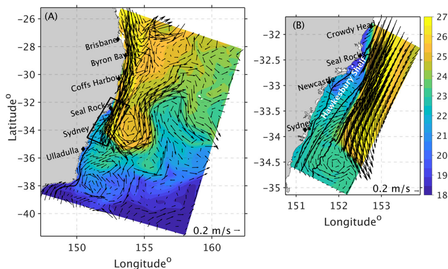
FIGURE 1 | Maps of sea surface temperature (°C) and surface velocity vectors along the east coast of Australia for 9th Jan 2013 shown in (A) the EAC-ROMS parent model domain described by Kerry et al. (2016), where the black rectangle shows the domain of the HSM model and the black solid line indicates the 2,000 m isobaths. (B) the HSM model domain described by Ribbat et al. (2020a,b) and the location of the Hawkesbury Shelf, black solid lines indicate the 100, 200, and 2,000 m isobaths. The black dot by the coast of Sydney indicates the position of the first coastal artificial reef (OAR).
