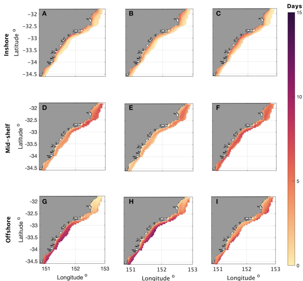
FIGURE 6 | Quantification of the number of days the water spent in each region across the shelf before arriving at the coast. i.e., the time spent inshore—between the coast and the 50 m isobath ( A–C ), over the mid-shelf, between the 50 and 100 m isobaths ( D–F ), and offshore, between the 100 m isobath and deeper ( G–I ), shown for each of the three case studies representing the 3 circulation modes ('EAC mode', 'EAC eddy mode', and 'Eddy dipole mode', respectively left to right). The number of days shown for each grid cell was computed as an average across all the particles released at each coastal grid cell.
