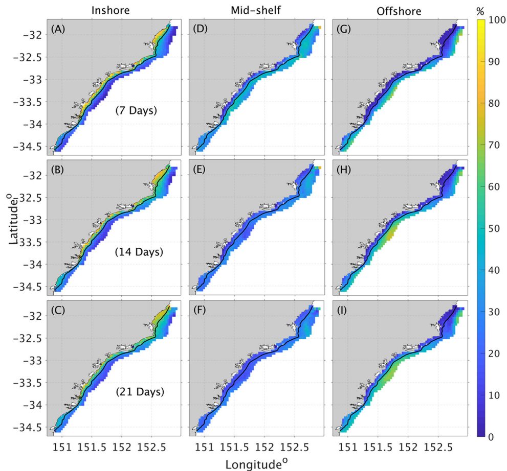
FIGURE 5 | Percentage of simulated particles arriving at each grid cell along the coastal (for particles released between the coast and the 100 m isobath) that come from: (A–C) , inner shelf region (0–50 m); (D–F) mid-shelf region (50–100 m) and (G–I) offshore region (>100 m) from 7, 14, and 21 days prior (top to bottom). The black solid line shows the 50 m isobath.
