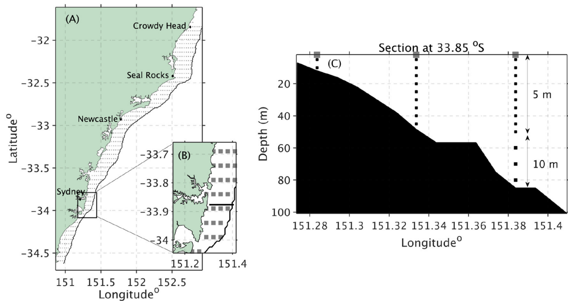
FIGURE 2 | Schematic diagram showing map of particle release locations. (A) Surface map of particle release sites along the HSM model domain. The grey squares show the release sites from the coast to the 100 m isobath. (B) Zoom in on the Sydney region to show the particle release positions and the location of the transect shown in (C) . (C) The depth structure of the releases across the inner shelf (black dots), particles are seeded every 5 m from the surface to 50 m, and 10 m from 50 to 100 m.
