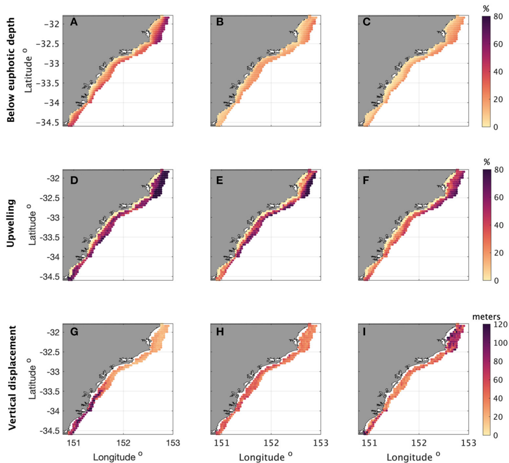
FIGURE 8 | Proportion of water that comes from (below the euphotic depth) (A–C); the proportion of water that was upwelled (D–F); and the mean vertical displacement (meters) of water parcels that were upwelled (G–I) for the three case studies, ‘EAC mode’ (left), ‘EAC eddy mode’ (middle), and ‘Eddy dipole mode’ (right) columns. The proportion of water below the euphotic depth was computed across particles released throughout the water column. The proportion of water that was upwelled was computed only considering the trajectories of particles that were released close to the sea floor.
