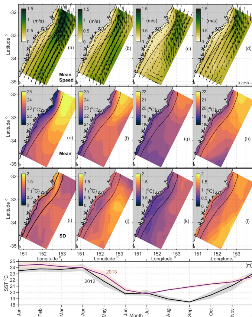
Fig 7. Domain-wide seasonal mean modelled fields. Velocity fields at the surface (a-d). Velocity vectors show the direction and colour shows the magnitude ( \text{ms}^{-1} ) of the speed. Every 25 th vector is shown for clarity. The reference velocity arrow in the bottom right of each panel represents 0.2 \text{ ms}^{-1} . Domain wide mean SST by season (e-h) and associated standard deviations (i-l) in ( ^{\circ}\text{C} ). Solid black lines show the 100 m and 2000 m isobaths. Area averaged SST (m) showing monthly means for 2012 (black), 2013 (red). Shaded areas represent the standard deviations.
