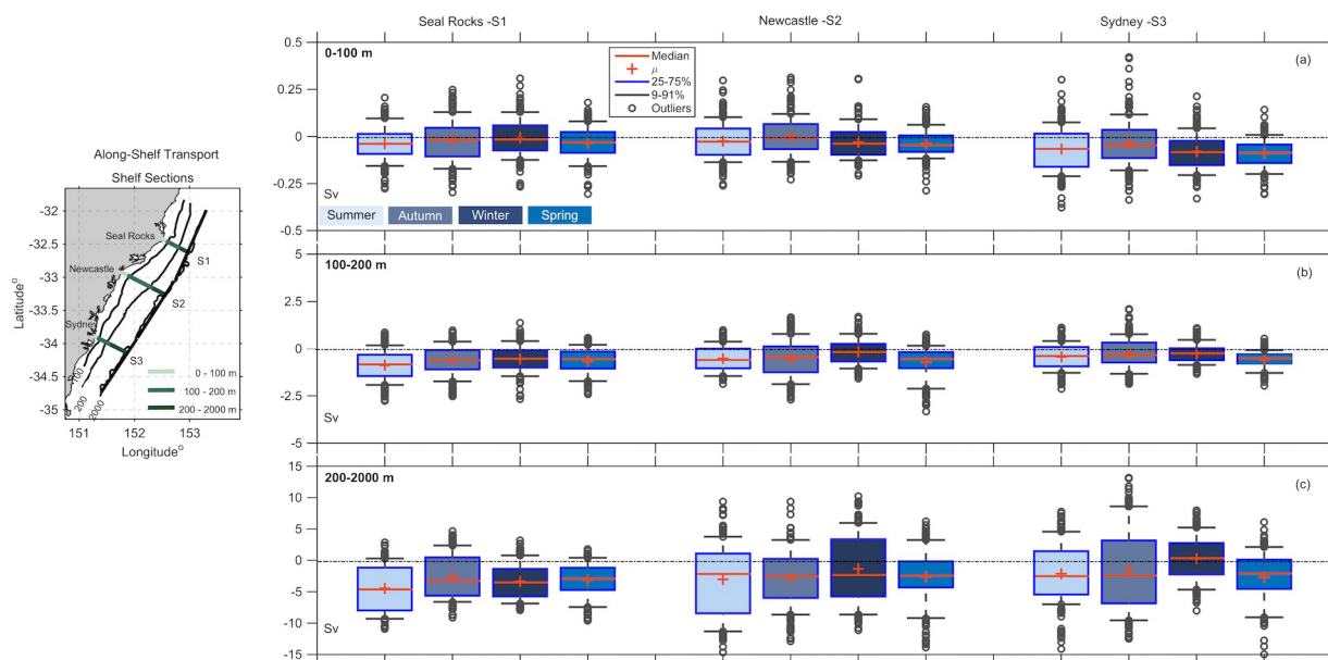
Fig 8. Box plots showing the along-shelf transport estimates ( S_v ) through three sections; Seal Rocks (S1), Newcastle (S2) and Sydney (S3), as shown in the map inset. The transports are shown across three segments a) the inner-shelf (0–100 m isobath) b) mid-shelf (100–200 m isobath), and c) across the outer shelf (200–2000 m isobath) coloured by season. Note the different scales for a, b, and c. As per the legend, the box plots show the median and the mean in red, the box shows the 25th to 75th percentiles, the tails show the 9th and 91st percentile, and the outliers are shown as circles.
