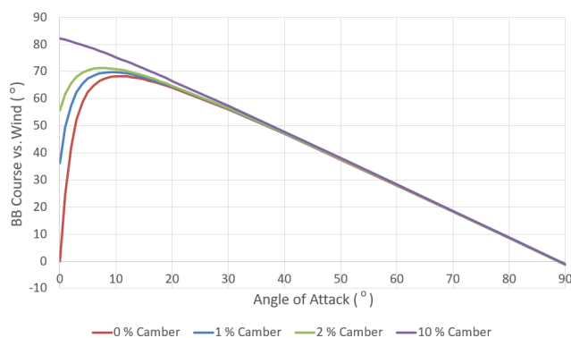
Figure 5. Bluebottle course relative to the wind ( 0^\circ means a downwind course) as a function of angle of attack ( 0^\circ means sail parallel to the wind) for different sail camber ratios.
