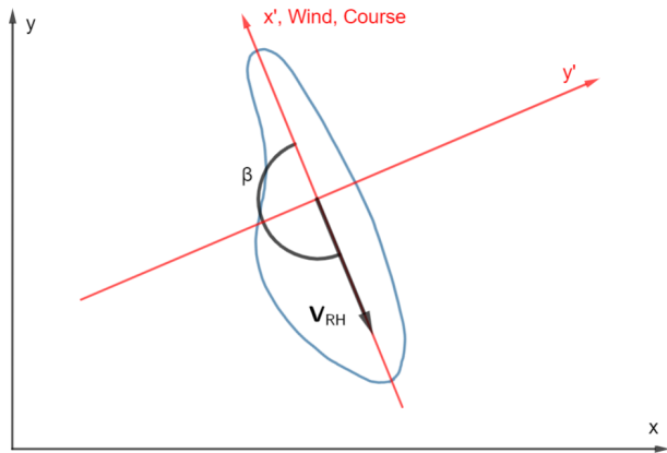
Figure 7. Case with no current for a left-handed (right-sailing) bluebottle sailing straight downwind with sail parallel to the wind direction ( \beta_a = 0^\circ ). Note that the wind direction and bluebottle course are on the x' axis. A right-handed (left-sailing) bluebottle would have the exact same course in this case.
