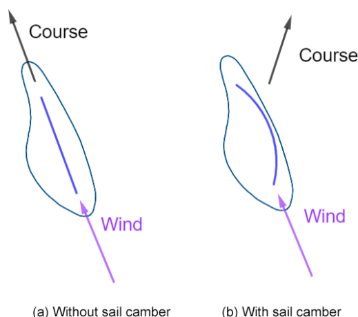
Figure 6. Bluebottle course at zero angle of attack is dependent on the sail camber. Panel (a) shows a bluebottle with no camber sailing straight downwind with sail parallel to the wind direction. Panel (b) shows a bluebottle with camber. Due to the curvature of the sail, even at zero angle of attack, the bluebottle course will diverge from the wind direction.
