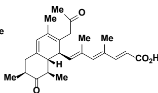
Embellistatin
