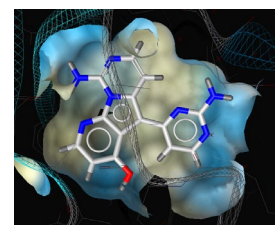
Variolin B
