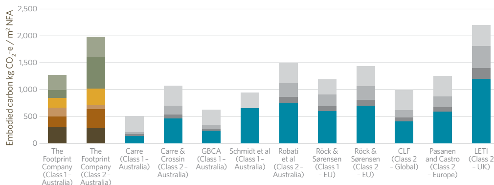
Figure 15: International residential (Class 1 & 2) embodied carbon benchmark (Average practice)
