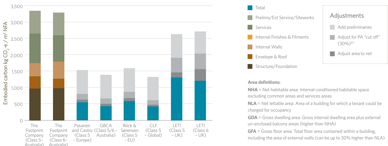
Figure 16: International residential (Class 5 & 6) embodied carbon benchmark (Average practice)
