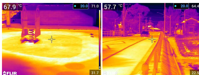
Figure 6. Infrared view of the playground and road in front of the Tregear Community Centre, reaching high surface temperatures during a summer afternoon, with a semi-hourly average outdoor air temperature of 35.3 \text{ }^{\circ}\text{C} measured on-site at 1.8 \text{ m} height and relative humidity of 27% (images taken in February 2022).
