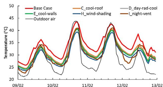
Figure 17. Indoor air temperatures in the hall, in the unretrofitted (base case) and retrofitted scenarios, computed during a historical heatwave event (February 2017). The solid black line displays the outdoor air temperature as measured at Horsley Park.
