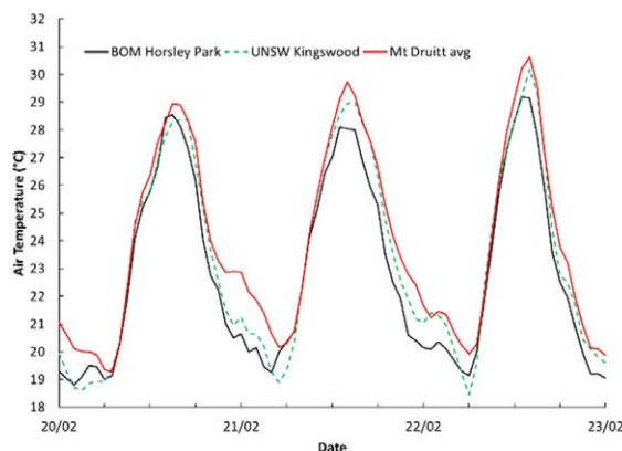
Figure 3. Ambient temperatures
