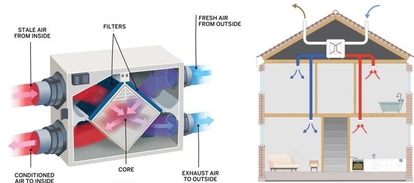
Figure 9: Centralised Mechanical Ventilation with Heat Recovery
