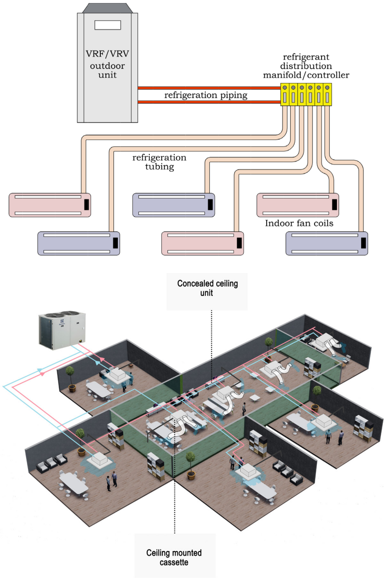
Figure 4: VRF/VRV system schematic diagram and typology
