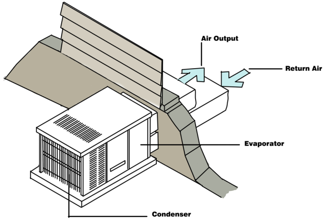
Figure 5: Unitary air-conditioner
