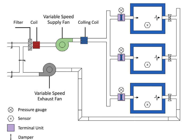
Figure 3: VAV system schematic diagram
