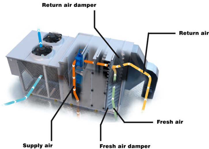
Figure 7: Packaged rooftop air-conditioner
