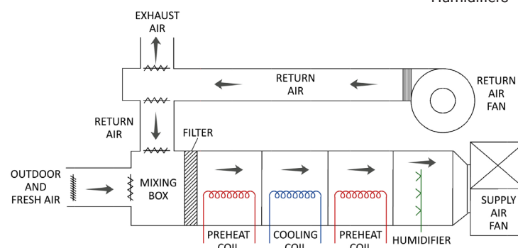
Figure 1: Schematic diagram of typical AHU
