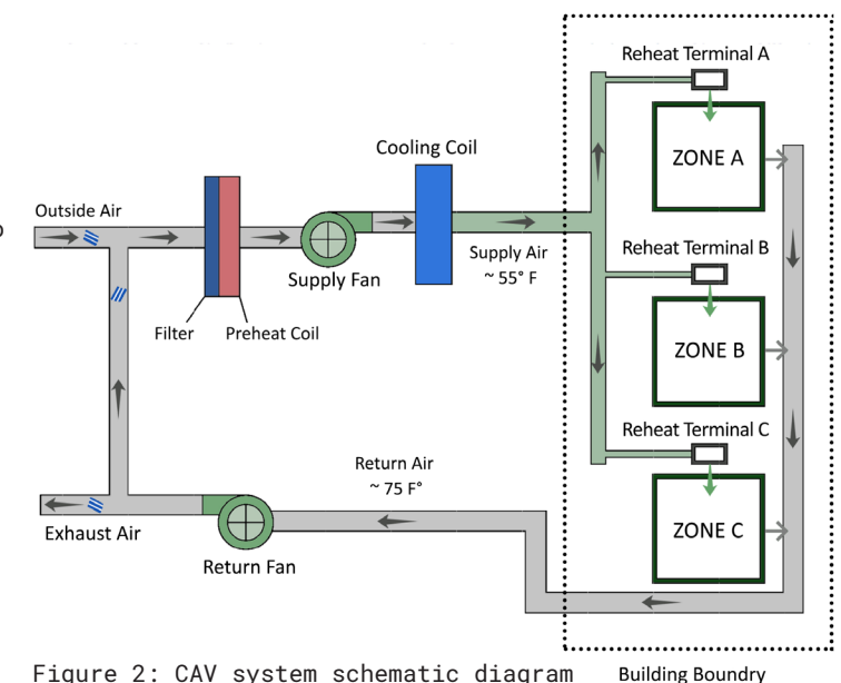
Figure 2: CAV system schematic diagram
