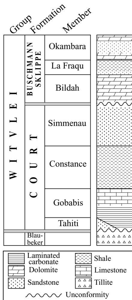
Fig. 2. Stratigraphy and idealised geological section of the Witvlei Group, Nama Basin, Namibia (after Hegenberger, 1993).
